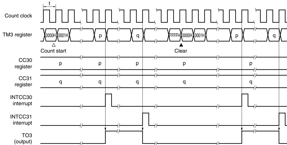
Figure 9-93. PWM Output Operation Timing Example
