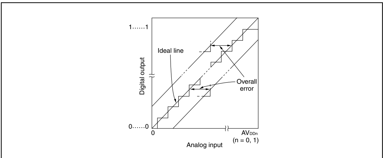
Figure 11-16. Overall Error
