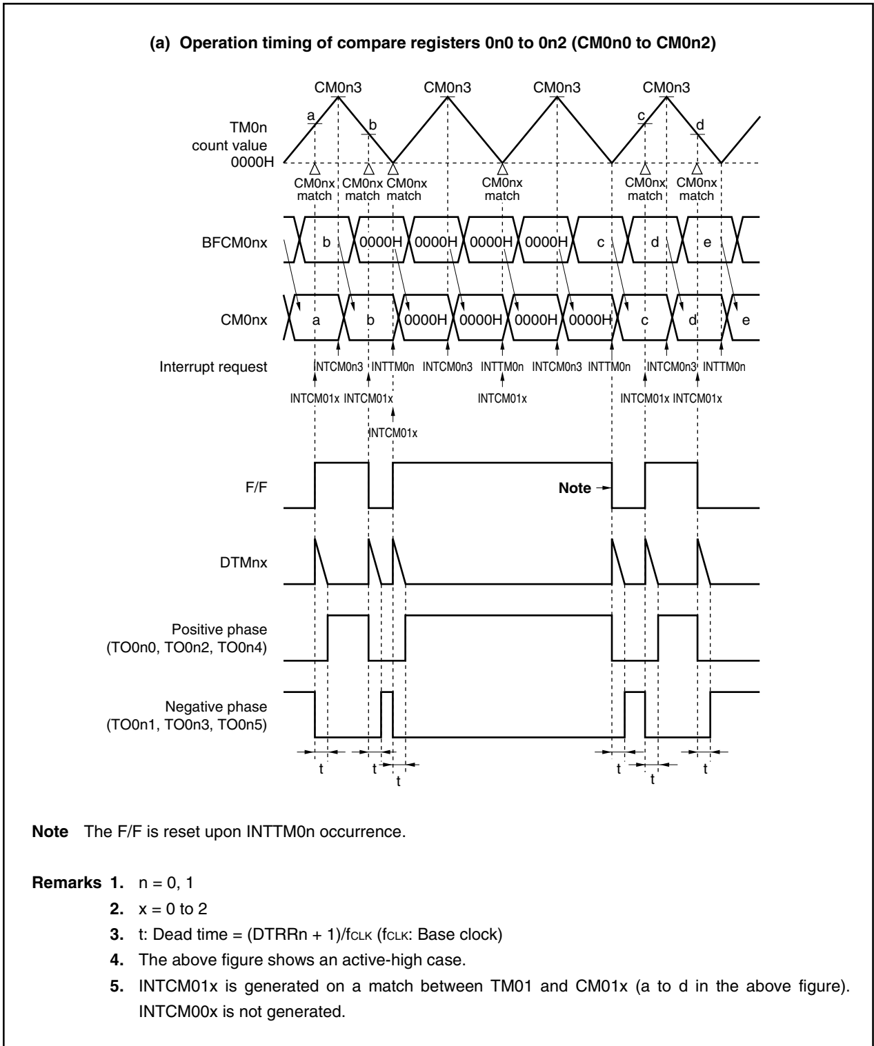
Figure 9-26. Change Timing from 100% Duty State (1) (PWM Mode 1) (1/2)
