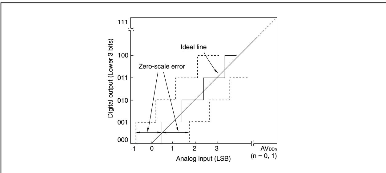
Figure 11-18. Zero-Scale Error
