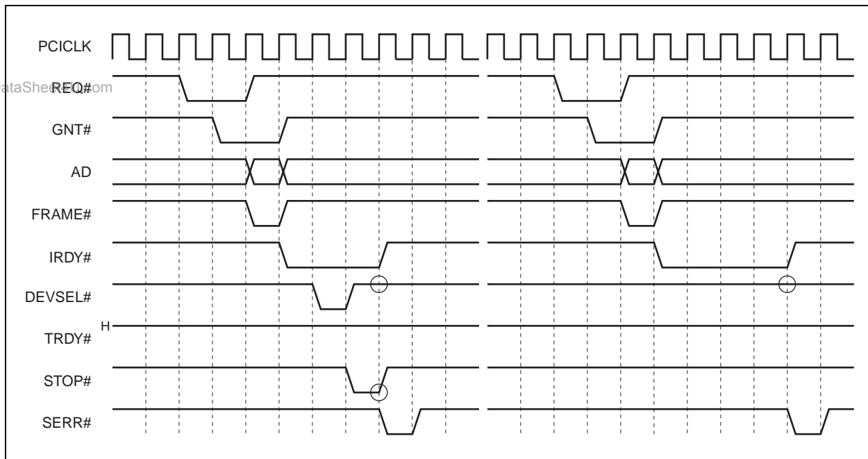
Figure 3-20. Abort Cycle
