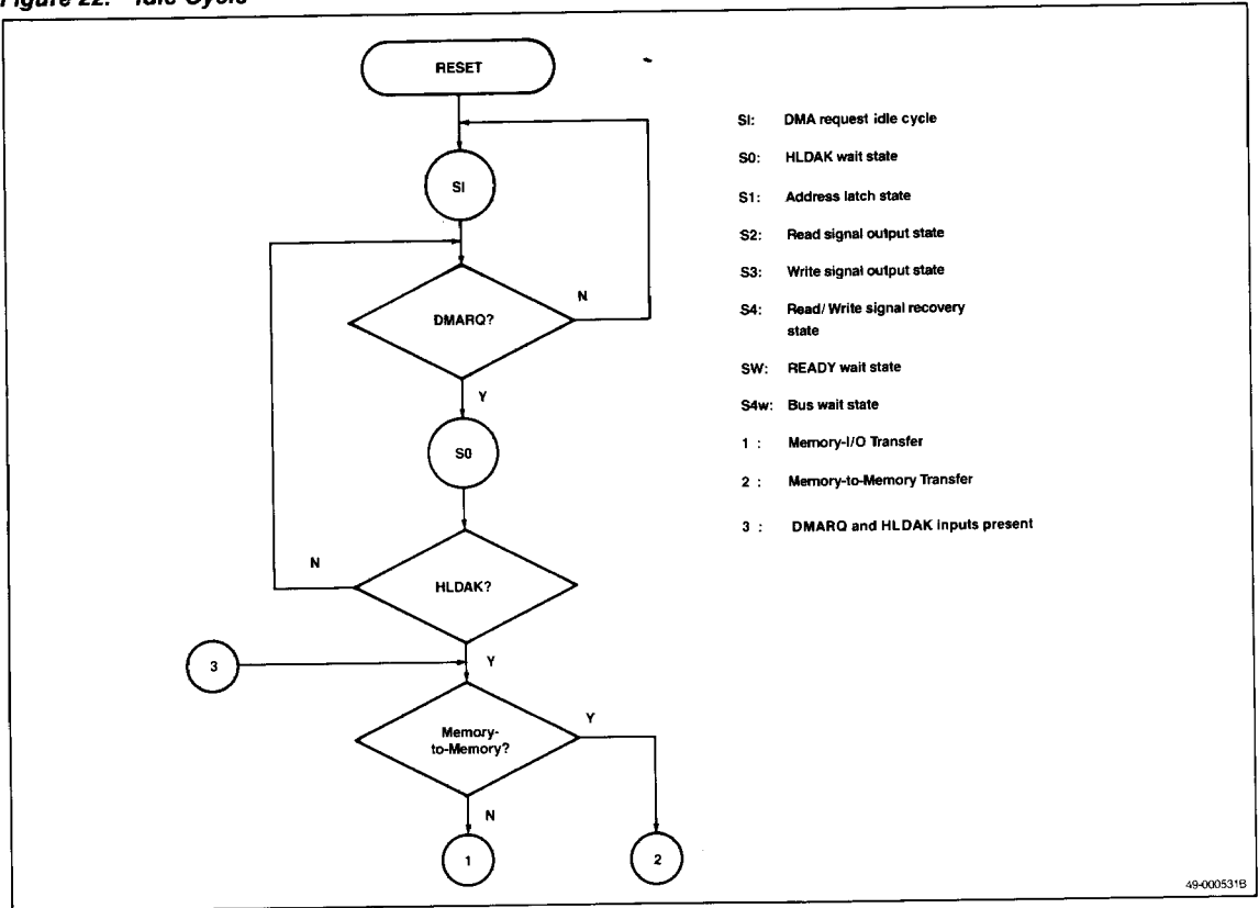
Figure 22. Idle Cycle
