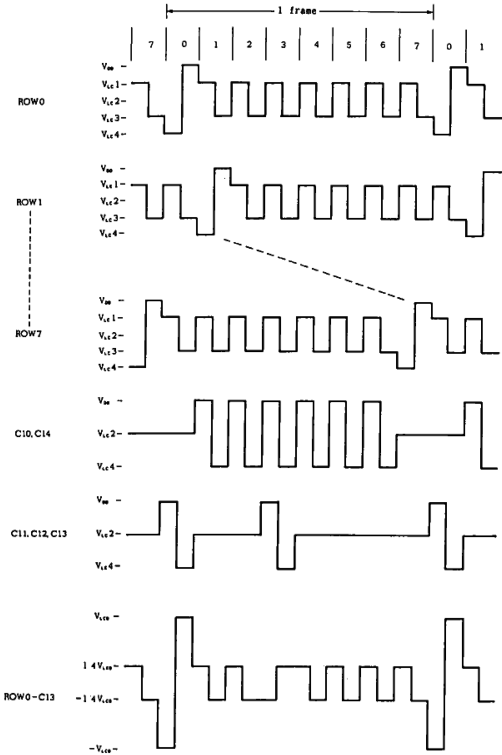
Fig. 6-2 8-Time-divisions (When Displaying Character A)
