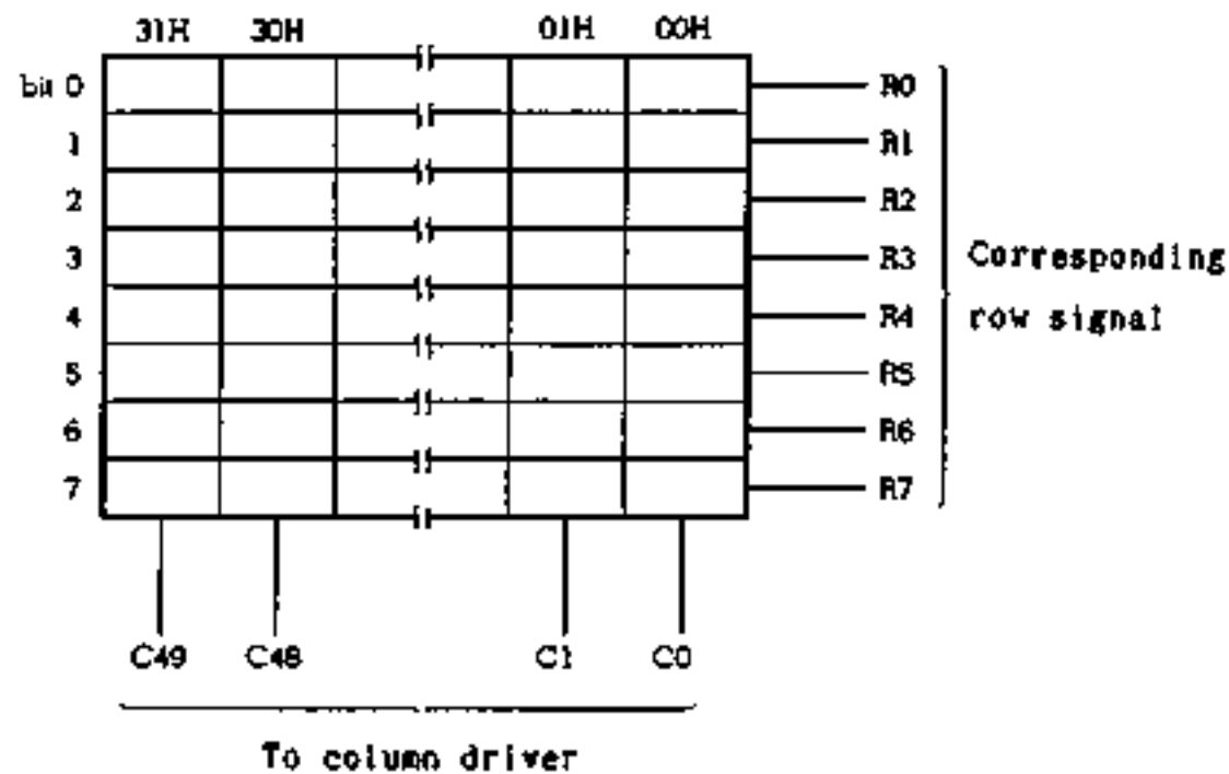
Fig. 2-6 Data Memory (8-Time-Division, Single/Multi-Chip)
