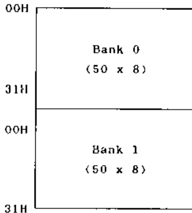
Fig. 2-5 Data Memory Configuration
