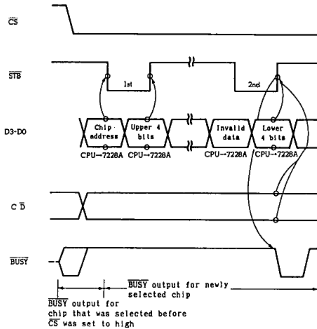
Fig. 3-5 Parallel Input Timing
