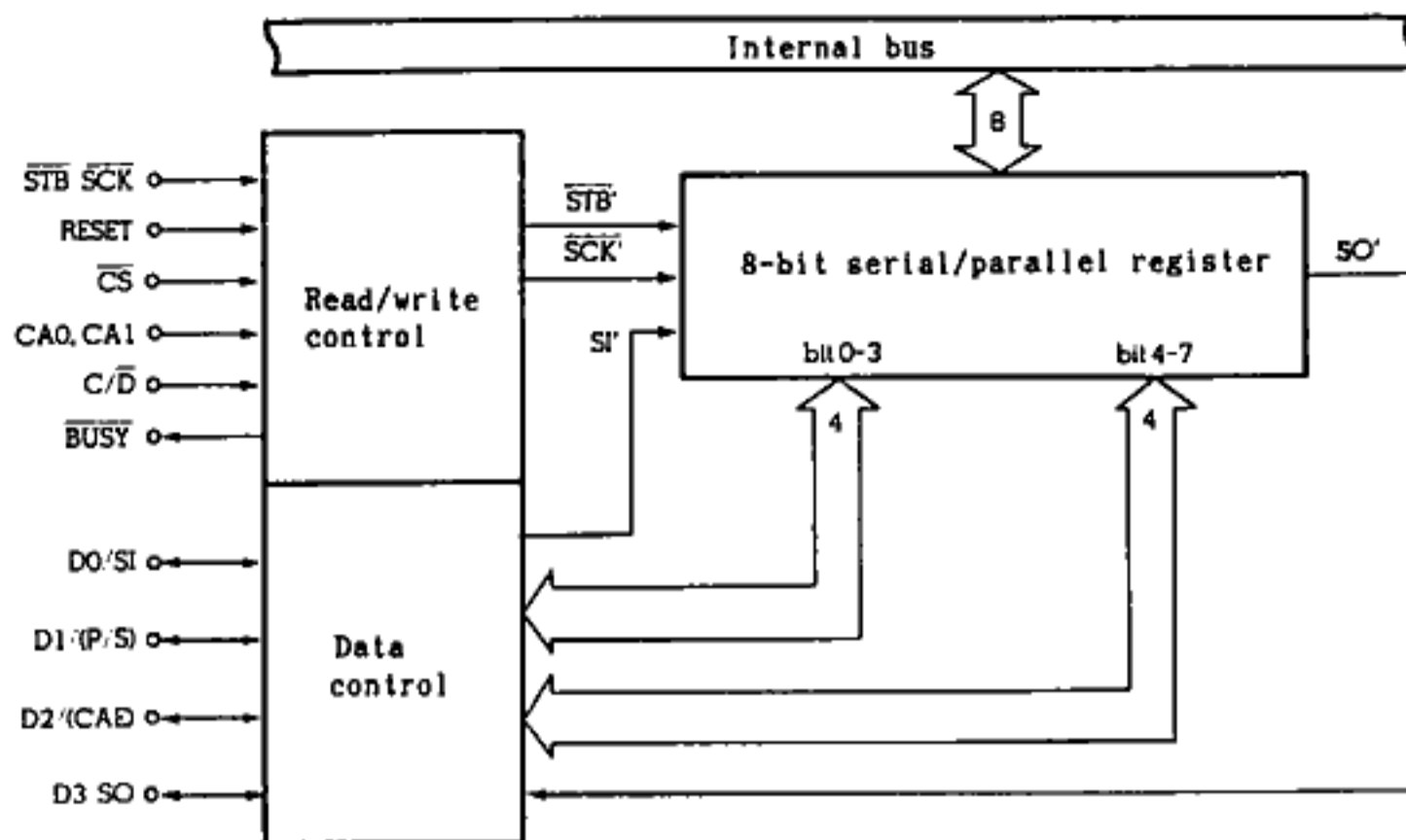
Fig. 2-1 Serial/Parallel Interface
