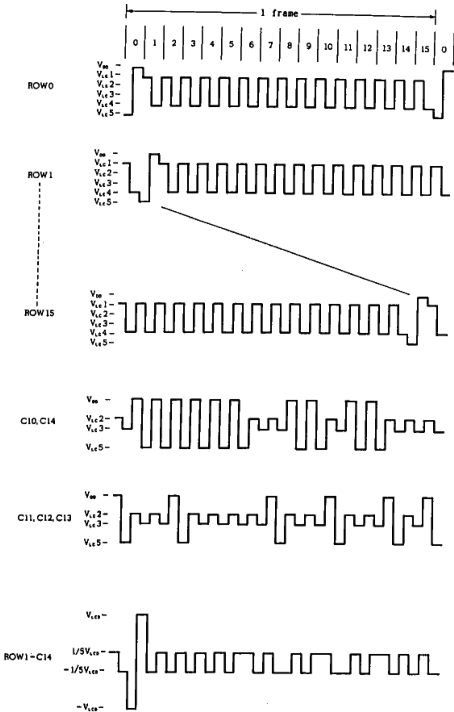
Fig. 6-4 16-Time-divisions (When Displaying Characters A and 8)
