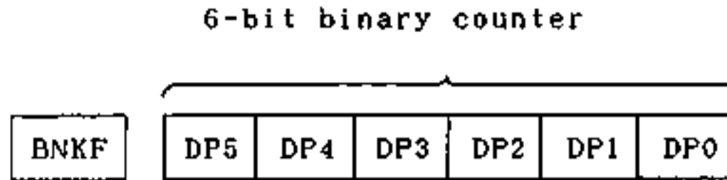
Fig. 2-4 Data Pointer Organization
