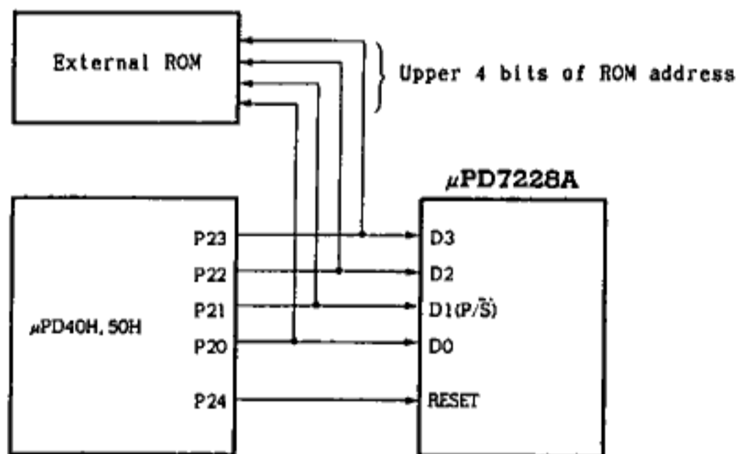
Fig. 10-3 Typical Connection When Using External ROM (Parallel Interface)
