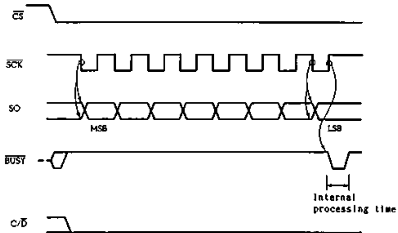
Fig. 3-2 Serial Output Timing Waveforms
