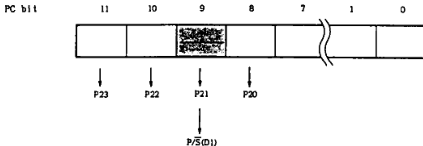
Fig. 10-4 Program Counter (PC) for uPD40H and uPD50H
