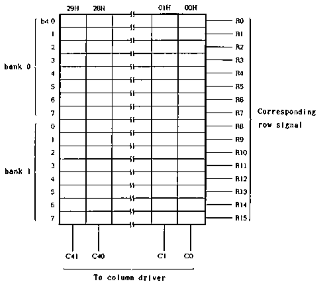
Fig. 2-7 Data Memory (16-Time-Division, Single-Chip)
