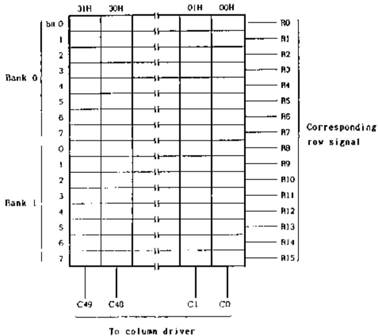
Fig. 2-8 Data Memory (16-Time-Division, Multi-Chip)
