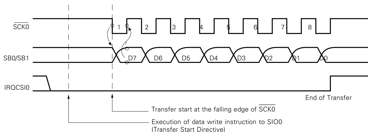
Fig. 4-51 2-Wire Serial I/O Mode Timing
