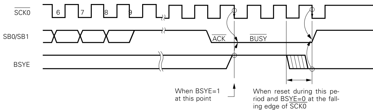
Fig. 4-48 BSYE Operation
