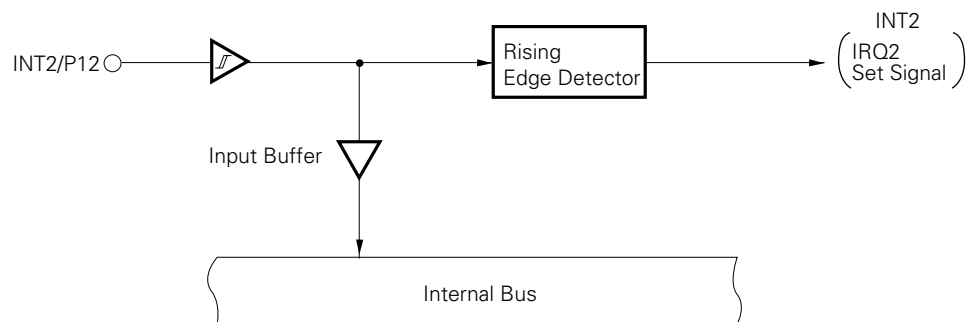
Fig. 5-3 INT2 Configuration
