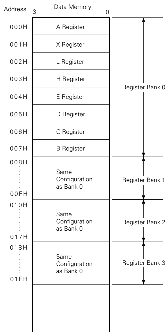
Fig. 3-5 General Register Configuraton
