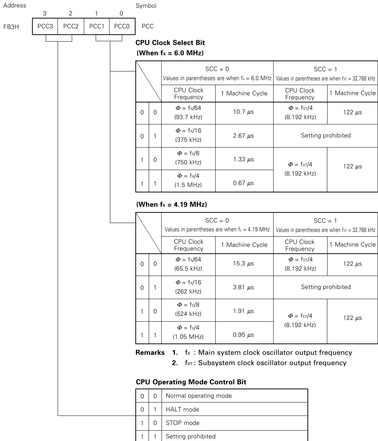
Fig. 4-15 Processor Clock Control Register Format
