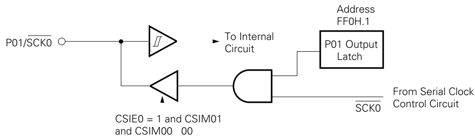
Fig. 4-58 \overline{\text{SCK0}} /P01 Pin Configuration
