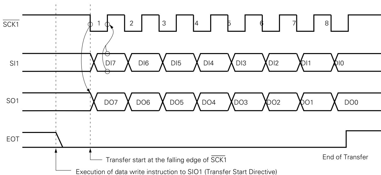
Fig. 4-61 3-Wire Serial I/O Mode Timing
