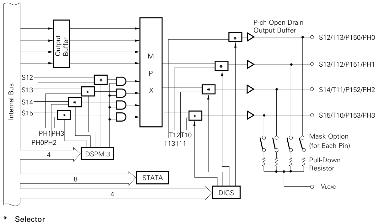
Fig. 4-11 Configurations of Ports 15 and H
