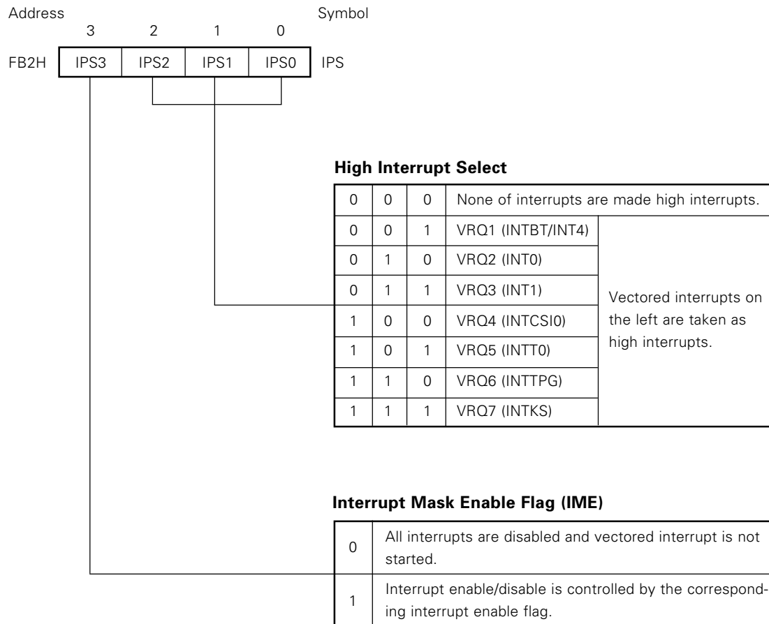
Fig. 5-5 Interrupt Priority Select Register
