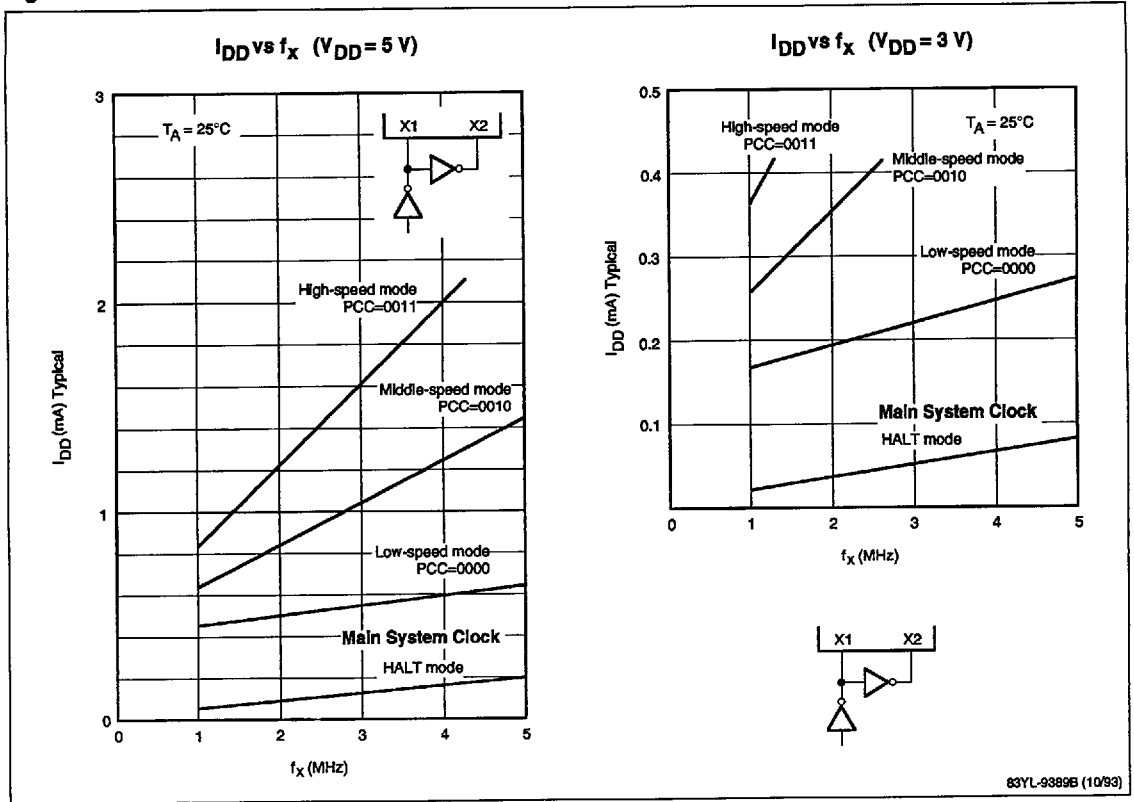
Figure 22. DC Characteristics, I_{DD} vs f_x (μPD7530x/31x, Standard Grade)
