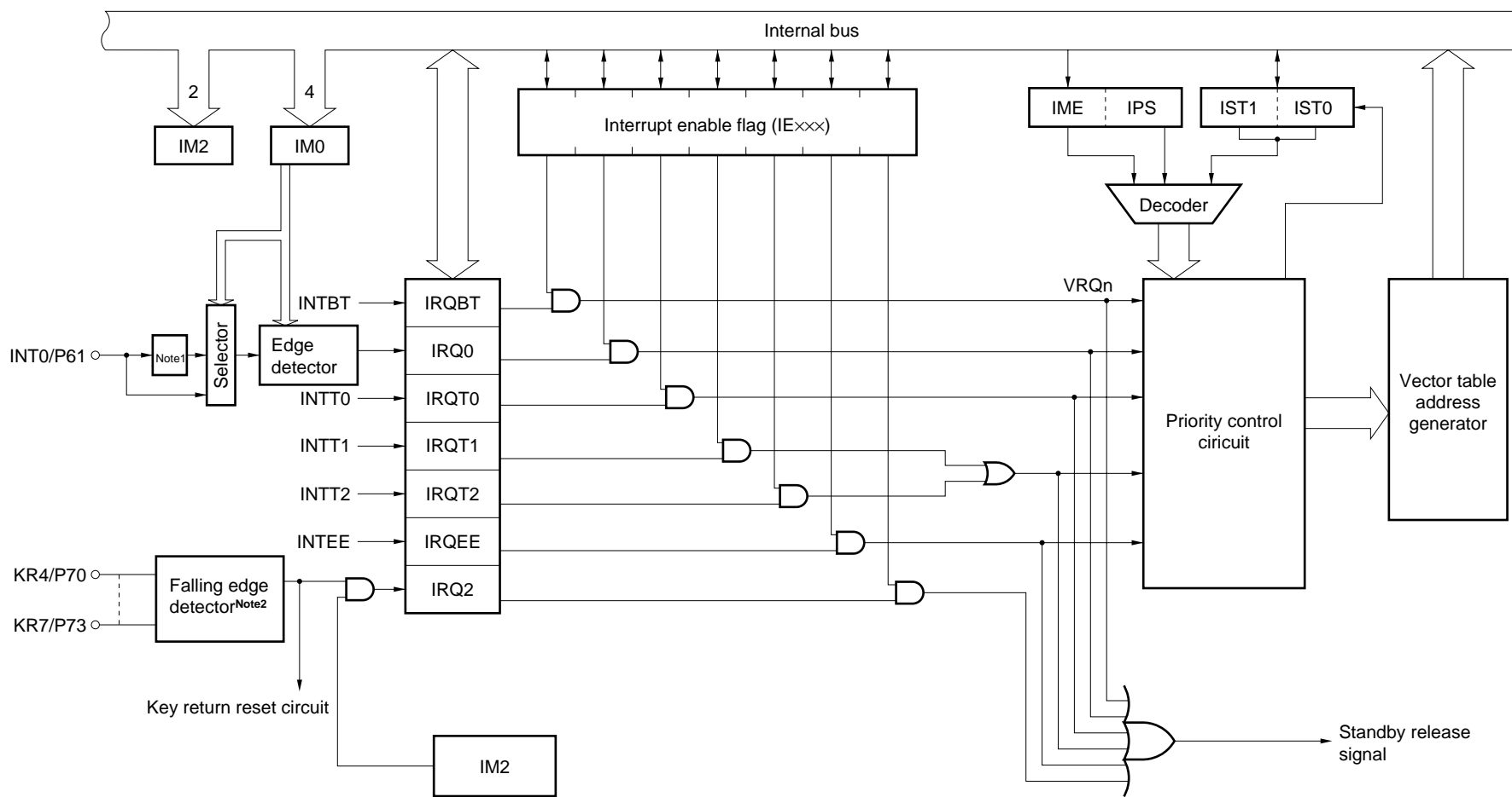
Figure 8-1. Interrupt Control Circuit Block Diagram
