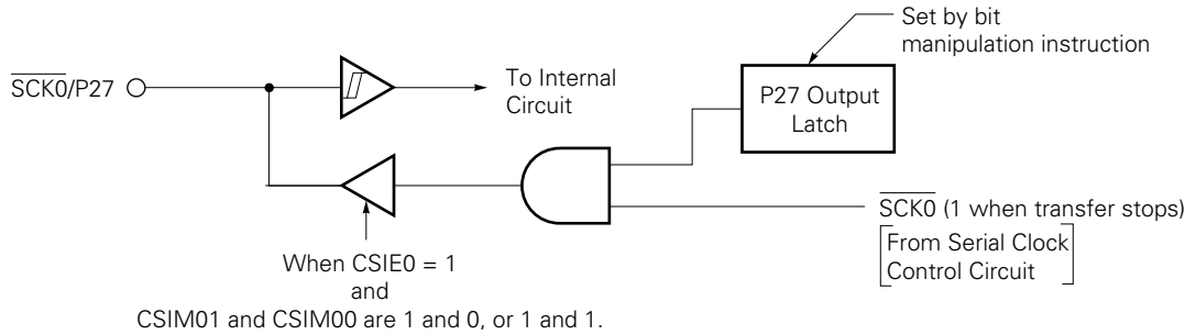
Figure 15-34. \overline{SCK0/P27} Pin Configuration
