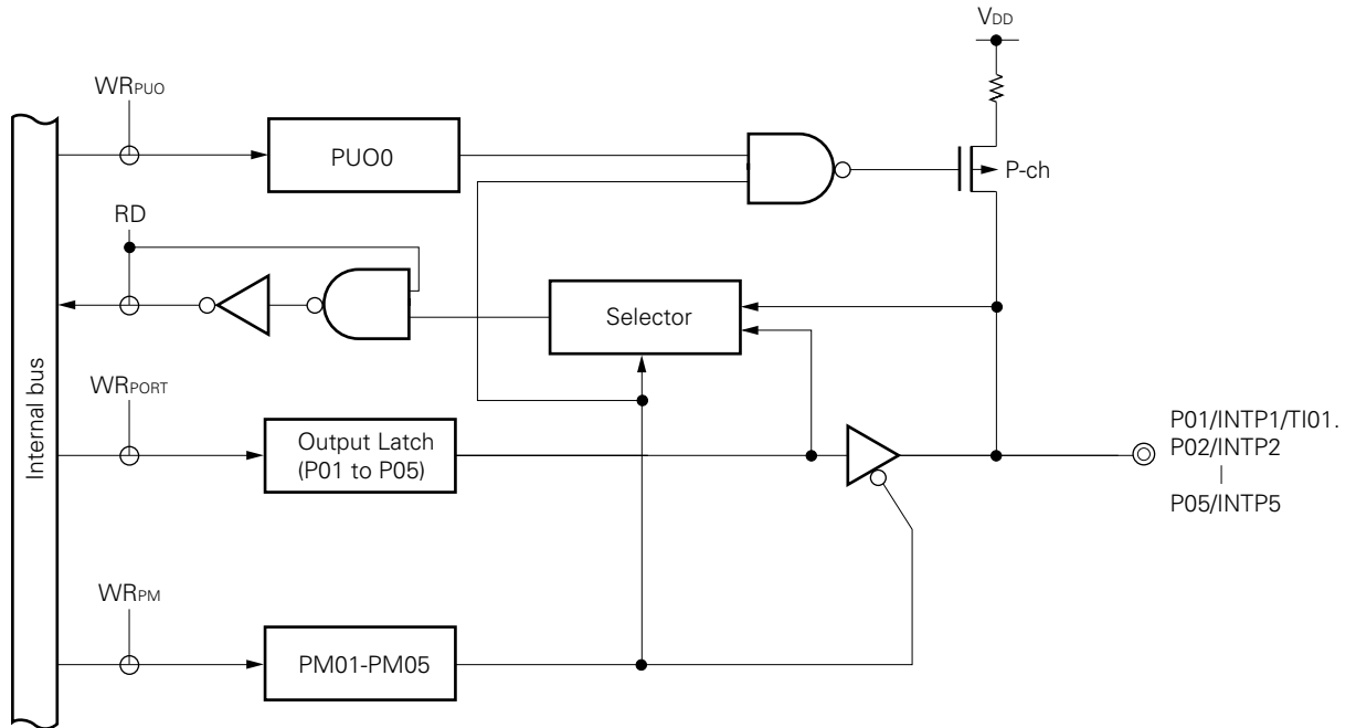
Figure 6-3. P01 to P05 Configurations
