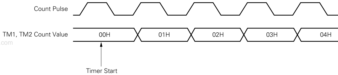
Figure 9-12. 8-Bit Timer Registers 1 and 2 Start Timing
