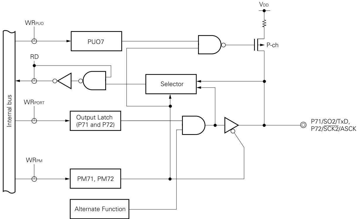
Figure 6-11. P71 and P72 Configurations
