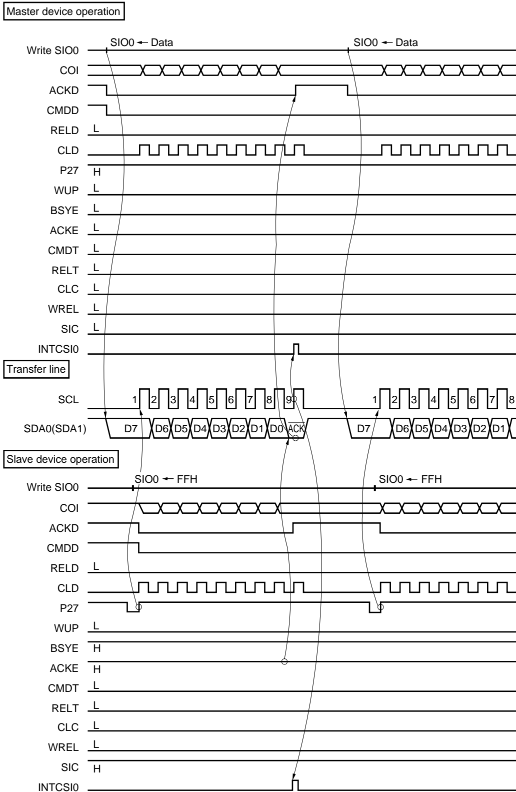
Figure 16-22. Data Transmission from Master to Slave (Both Master and Slave Selected 9-Clock Wait) (2 of 3) (b) Data
