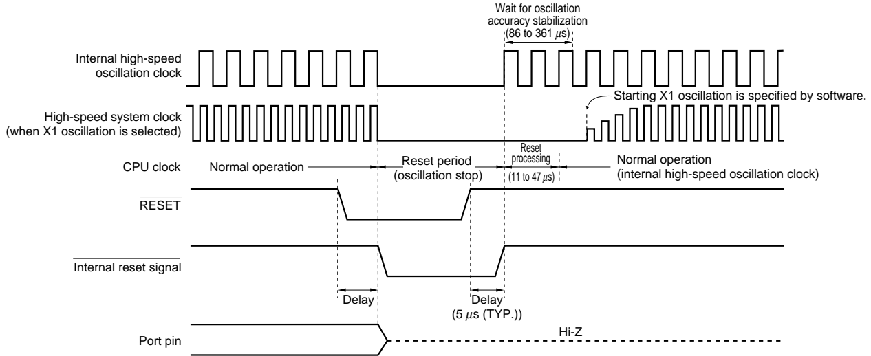
Figure 20-2. Timing of Reset by RESET Input
