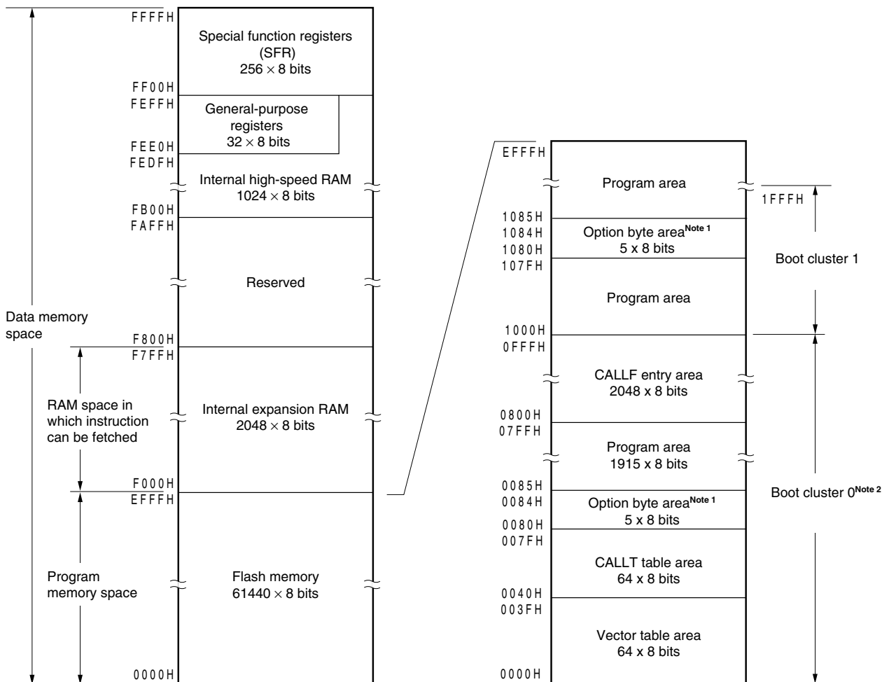
Figure 3-6. Memory Map ( \mu PD78F0515)
