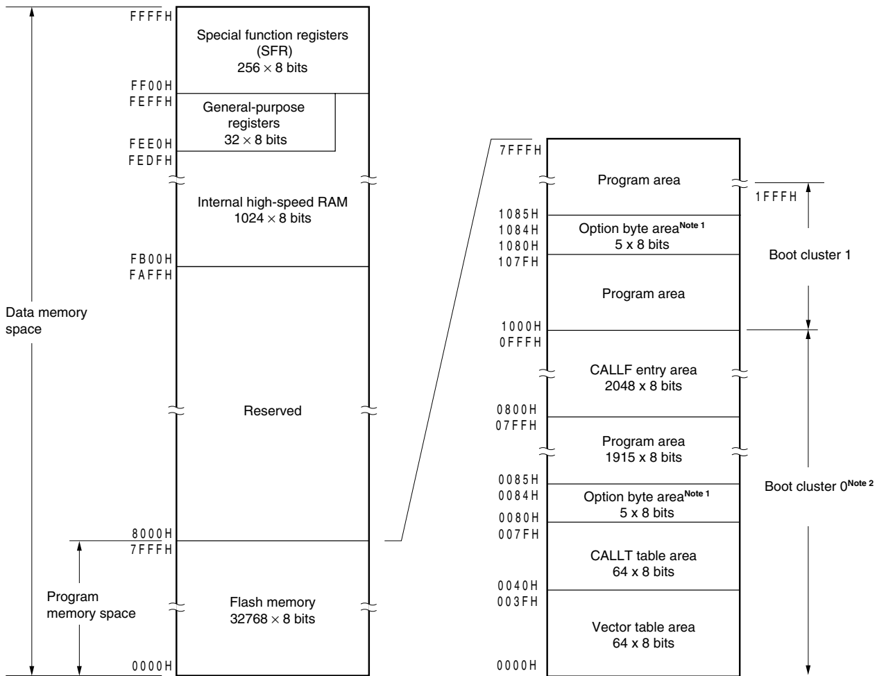
Figure 3-3. Memory Map ( \mu PD78F0513)
