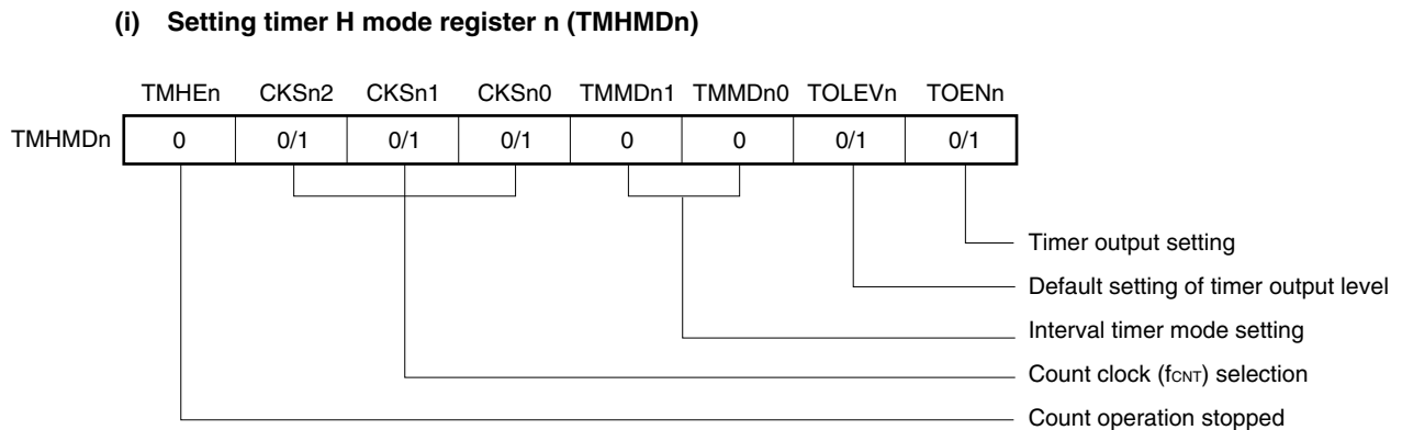
Figure 8-9. Register Setting During Interval Timer/Square-Wave Output Operation
