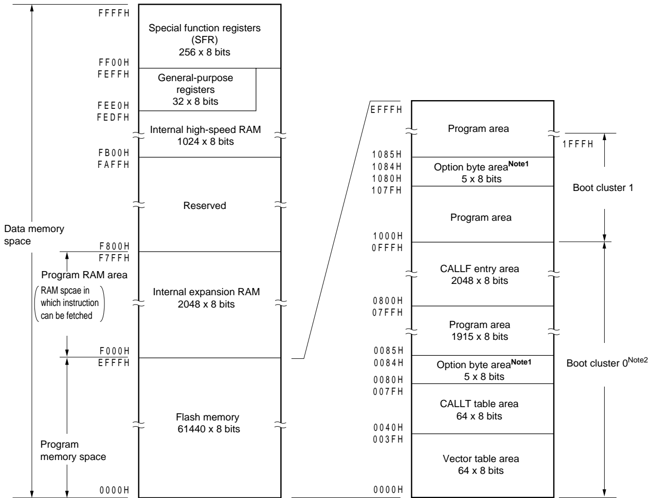
Figure 3-5. Memory Map (μPD78F0525)
