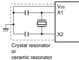
Figure 6-9. Example of External Circuit of X1 Oscillator (Crystal or Ceramic Oscillation)
