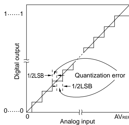
Figure 13-15. Quantization Error
