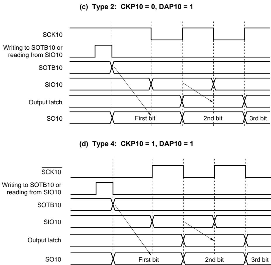
Figure 16-7. Output Operation of First Bit (2/2)
