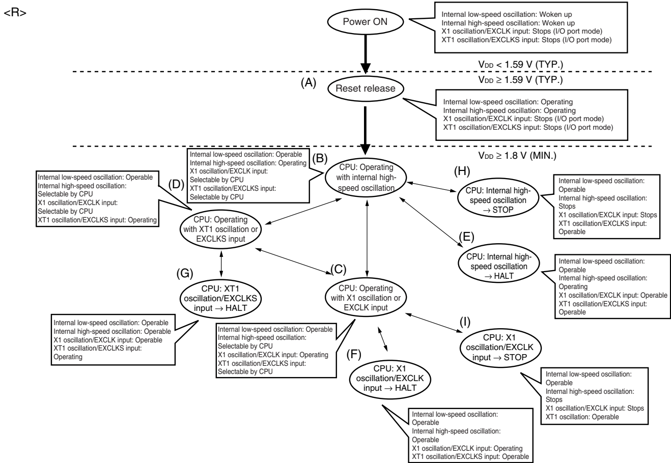
Figure 5-14. CPU Clock Status Transition Diagram
