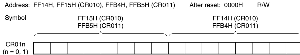
Figure 6-6. Format of 16-Bit Timer Capture/Compare Register 01n (CR01n)
