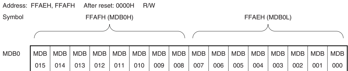
Figure 19-4. Format of Multiplication/Division Data Register B0 (MDB0)
