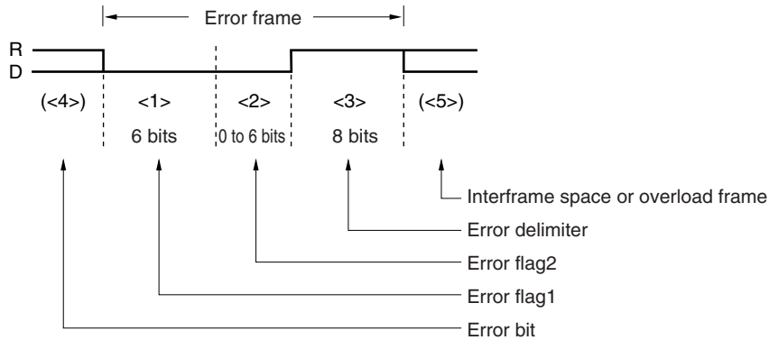
Figure 15-15. Error Frame
