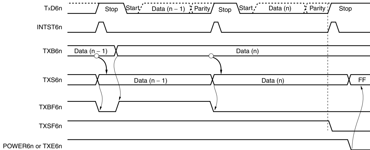
Figure 13-26. Timing of Ending Continuous Transmission
