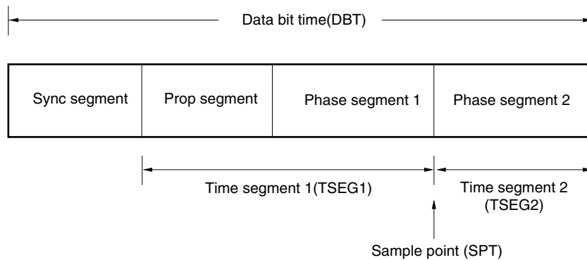
Figure 15-18. Segment Setting
