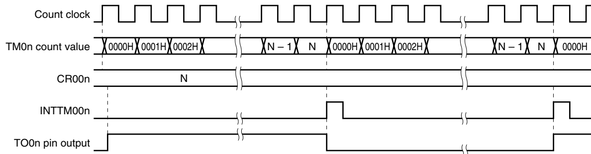
Figure 6-37. Square-Wave Output Operation Timing
