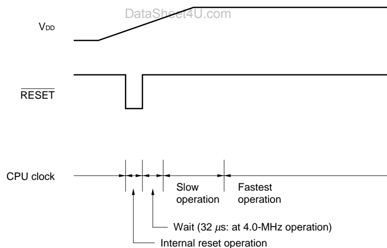
Figure 7-5. Switching CPU Clock
