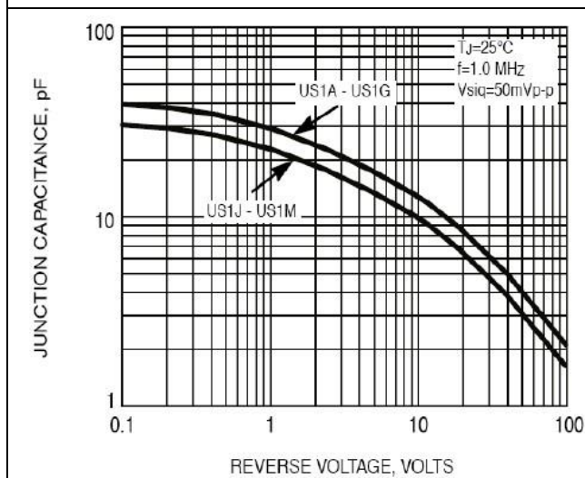
FIG. 5 TYPICAL JUNCTION CHARACTERISTICS
