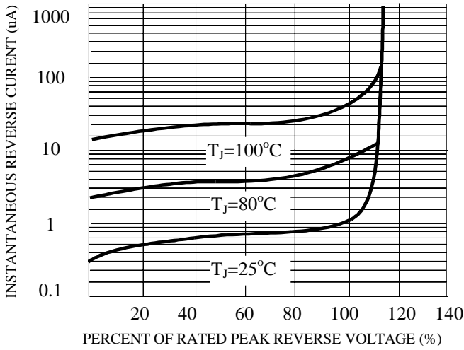
FIG. 3-TYPICAL REVERSE CHARACTERISTICS
