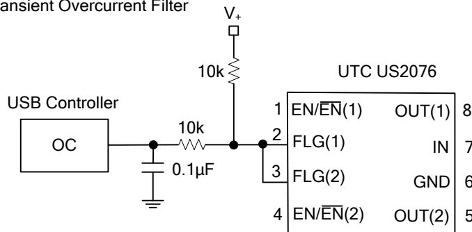
Transient Overcurrent Filter
