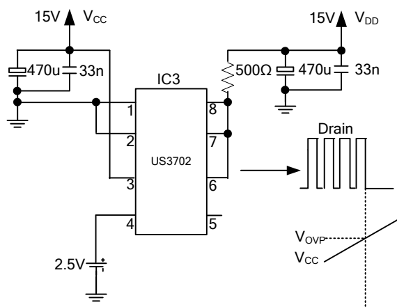
Fig.9 OVP test circuit
