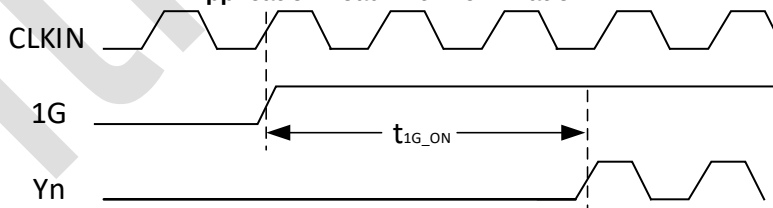
T_{1G\_ON} Output Enable Time
