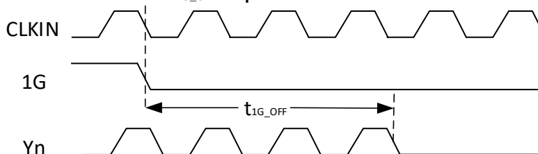
T_{1G\_OFF} Output Enable Time
