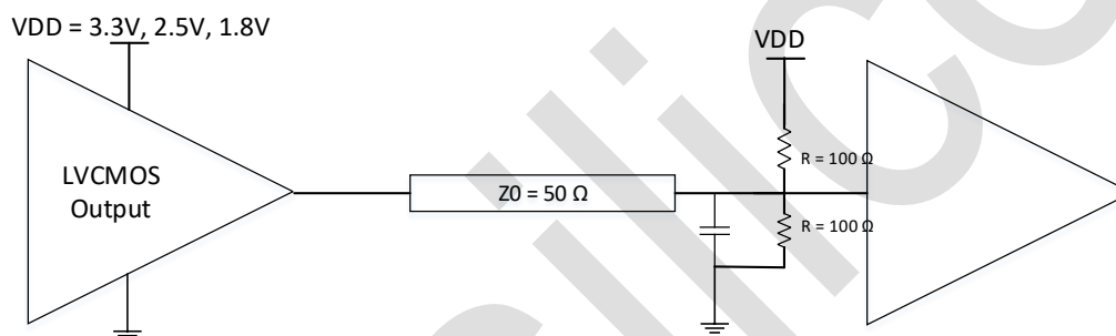
Application Load With 50- \Omega Termination
