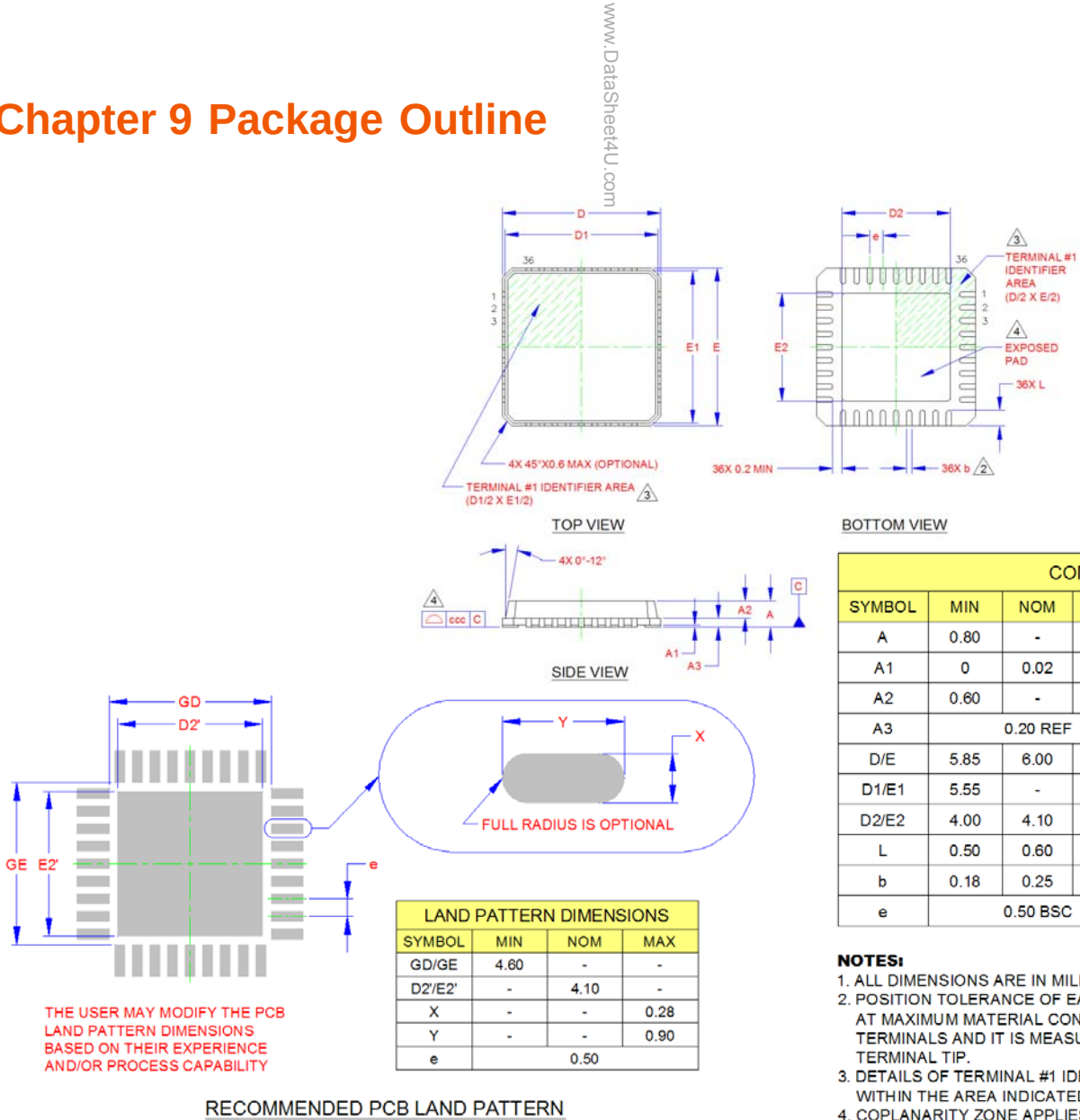
Figure 9.1 USB2244/USB2244i 36-QFN, 6x6mm Body, 0.5mm Pitch
