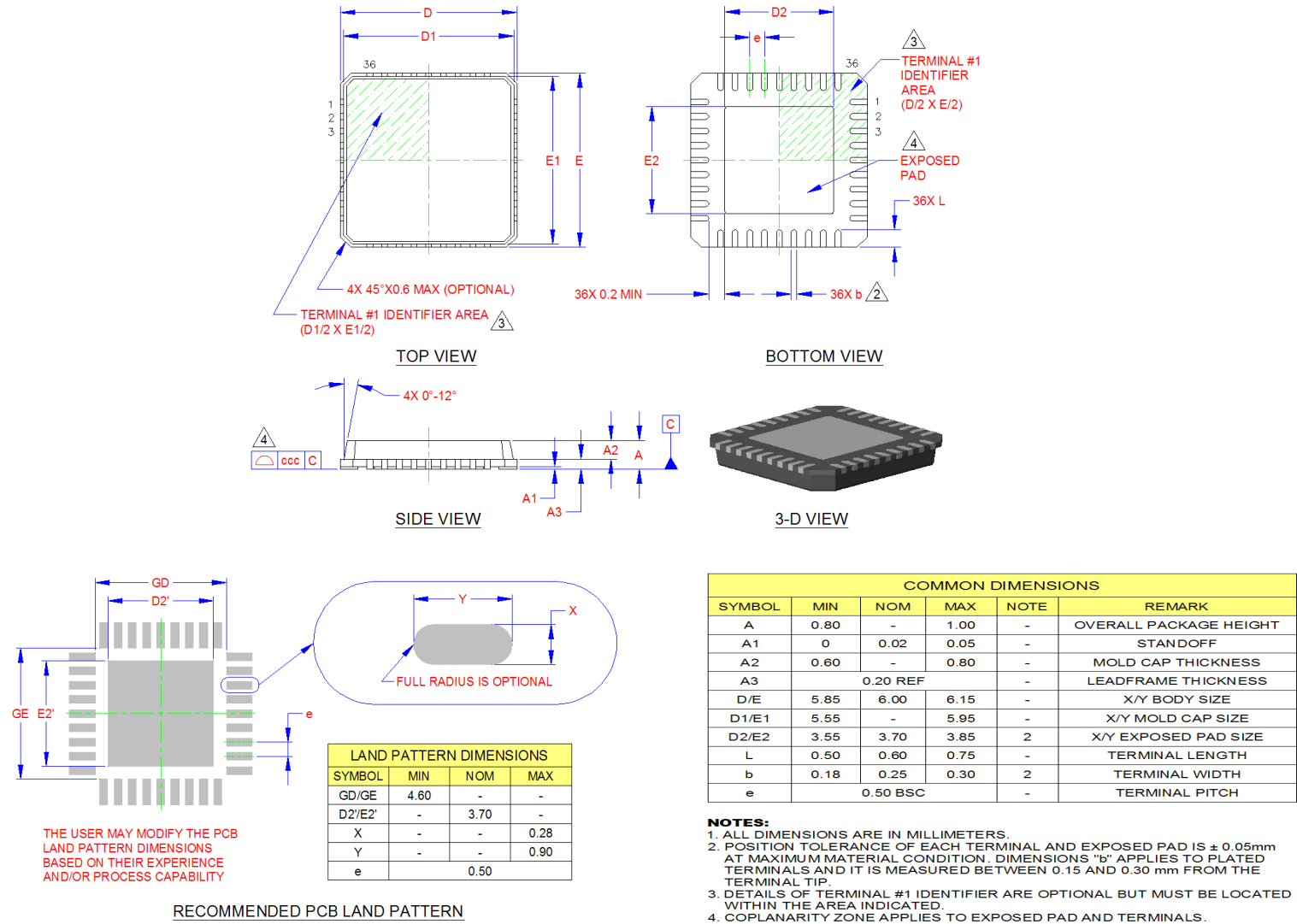
Figure 7.1 36-Pin QFN, 6x6mm Body, 0.5mm Pitch
