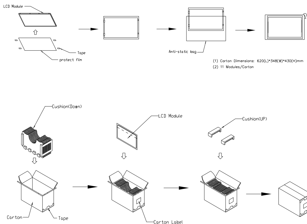
Figure. 7-1 Packing method
