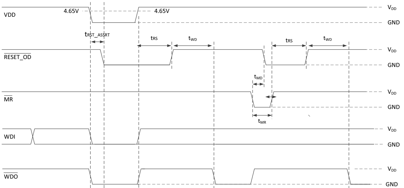
Figure 4. \overline{\text{RESET\_OD}} and \overline{\text{WDO}} are driven low for V_{DD} < 4.65 volts. \overline{\text{WDO}} is driven high when \overline{\text{MR}} is low
