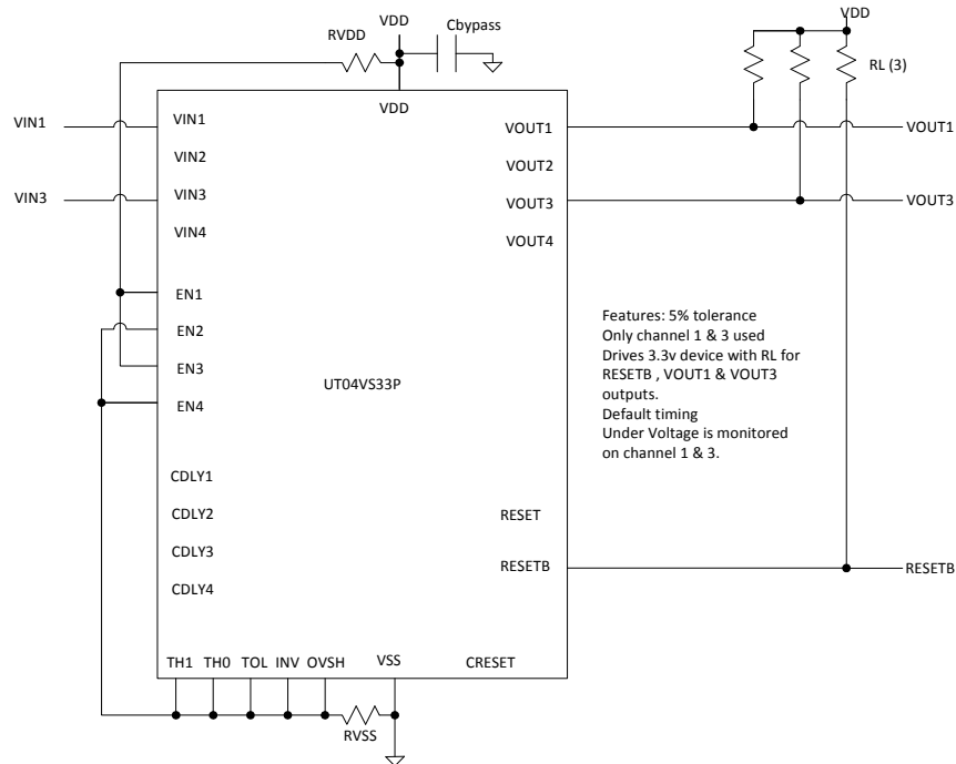
Figure 7. Application example of basic connection
