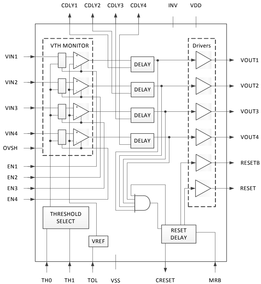
Figure 1. UT04VS33P Block Diagram
