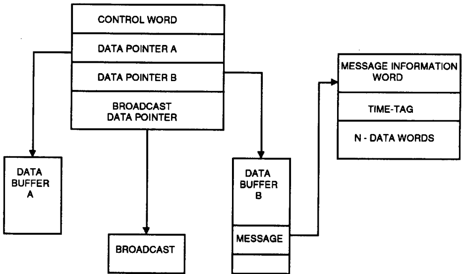
Figure 6. SRT Descriptor Block (Receive)
