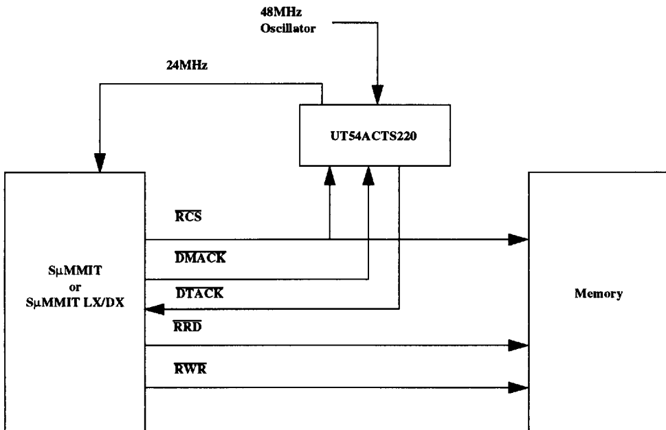
Figure 26. Wait-State Configuration using UT54ACTS220
