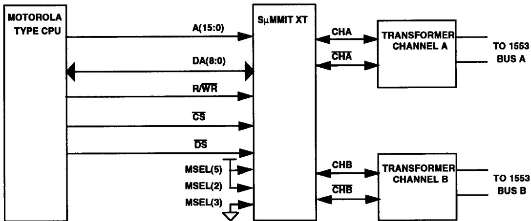
Figure 28b. 16-bit Interface (Motorola Type)
