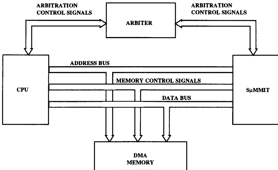
Figure 25. DMA System Configuration
