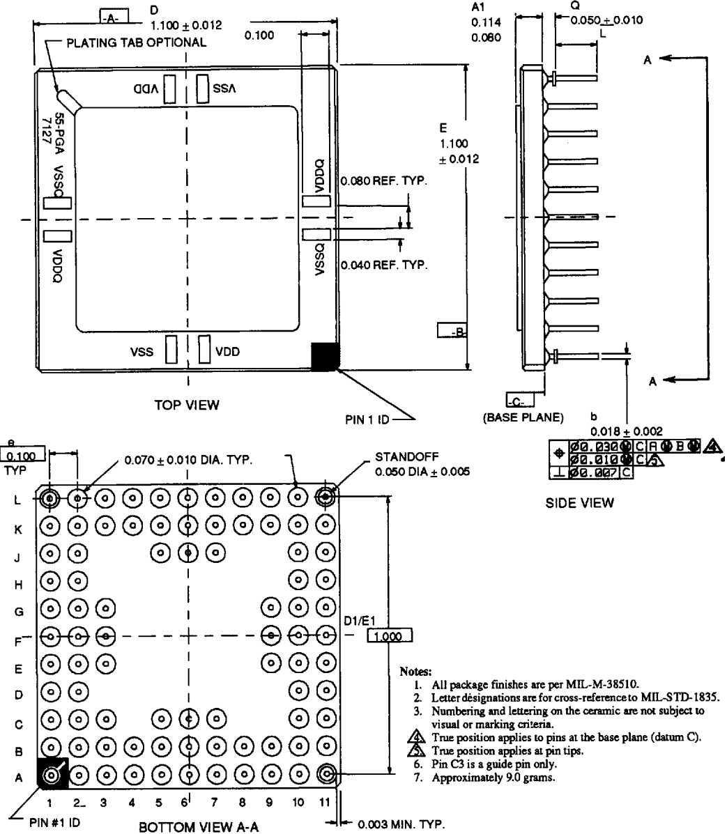
Figure 55. SμMMIT 85-Pin Pingrid Array
