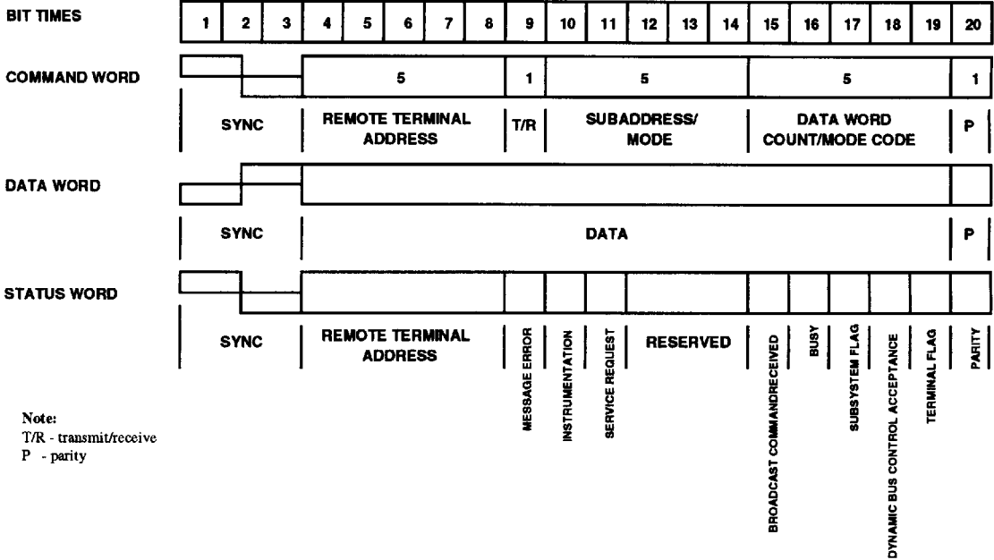
Figure 33. MIL-STD-1553B Word Formats
