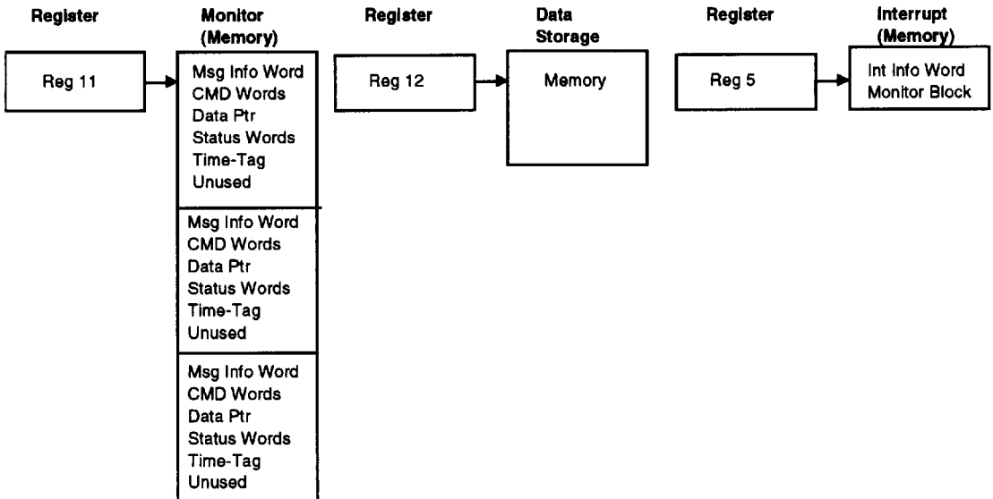
Figure 14. Memory Architecture for Monitor Mode
