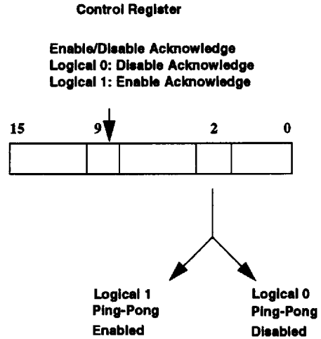
Figure 19. Ping-Pong Handshake
