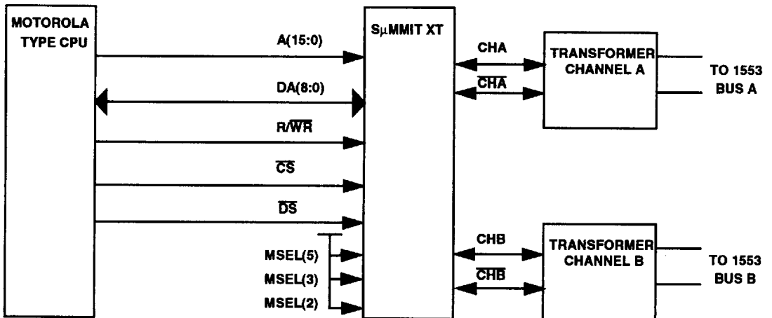
Figure 28d. 8-bit Interface (Motorola Type)
