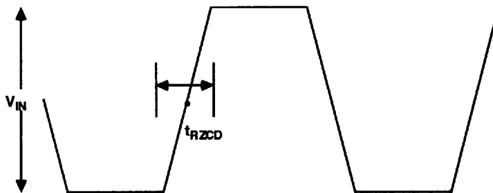
Figure 54. Receiver Input Zero Crossing Distortion ( t_{RZCD} )
