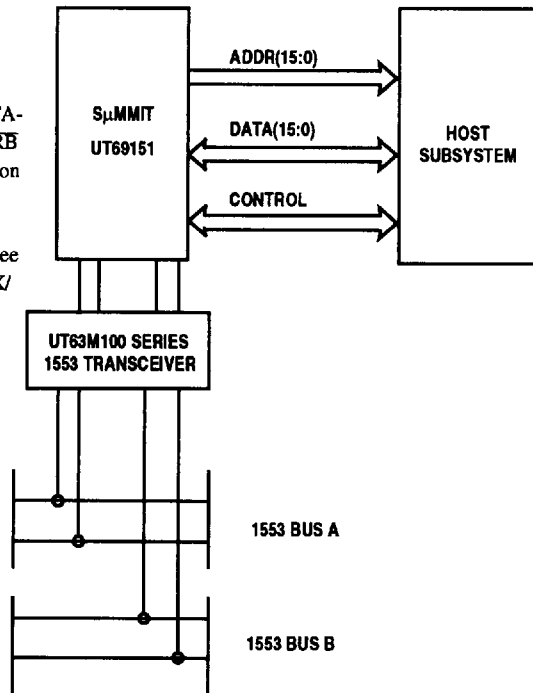
Figure 24a. S \mu MMIT General System Diagram
