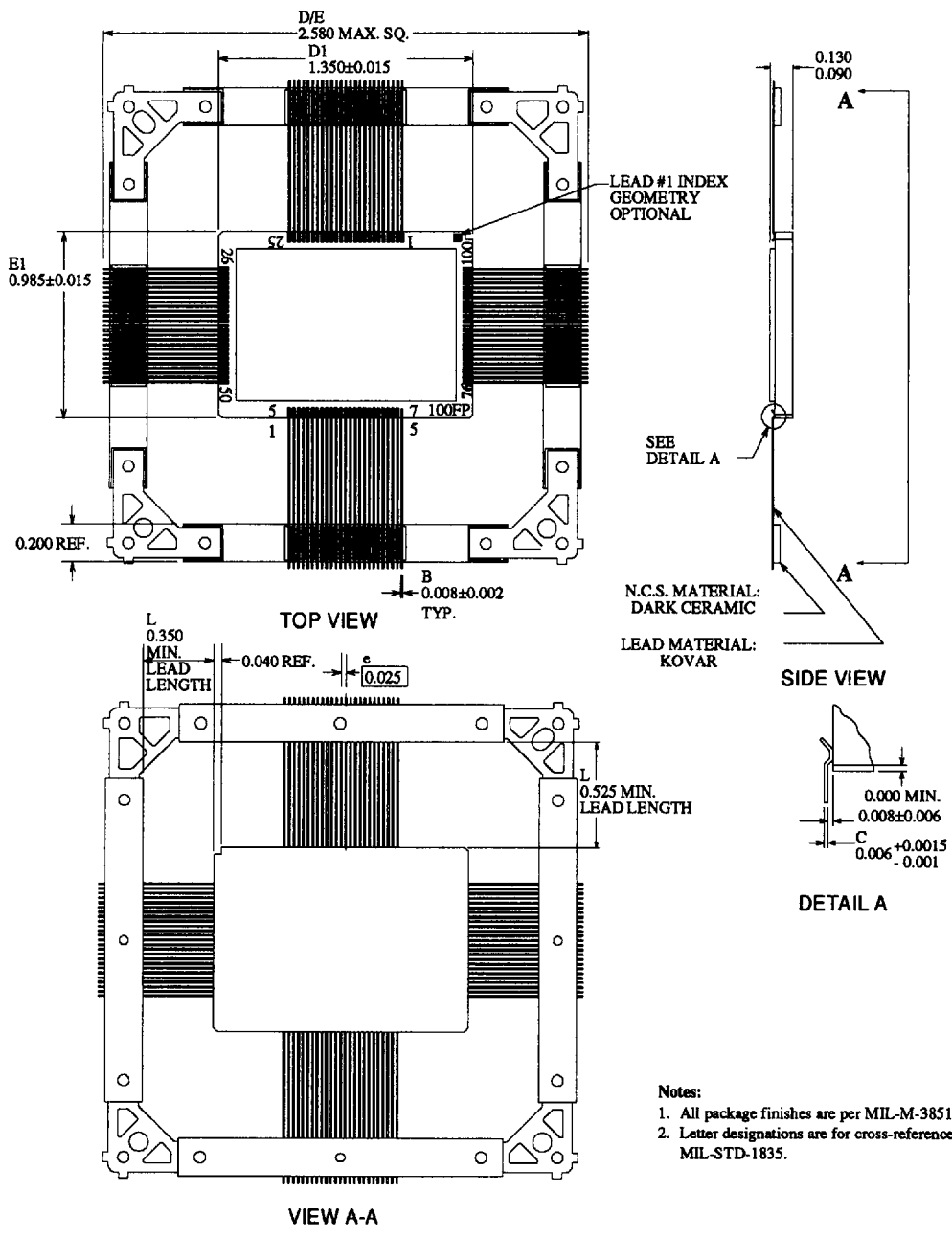
Figure 59. \mu MMIT LX/DX 100-Lead Flatpack
