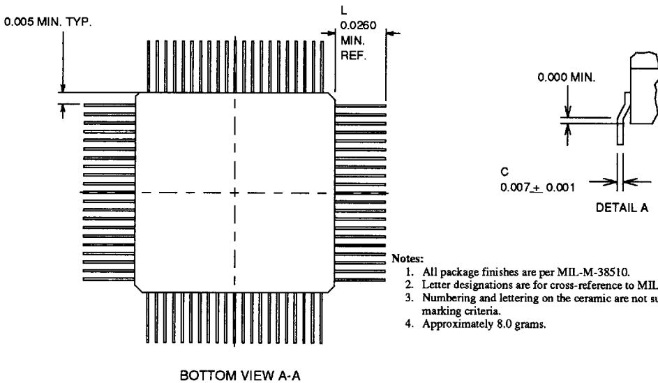
Figure 56. SμMMIT 84-Lead Flatpack (50mil lead spacing)
