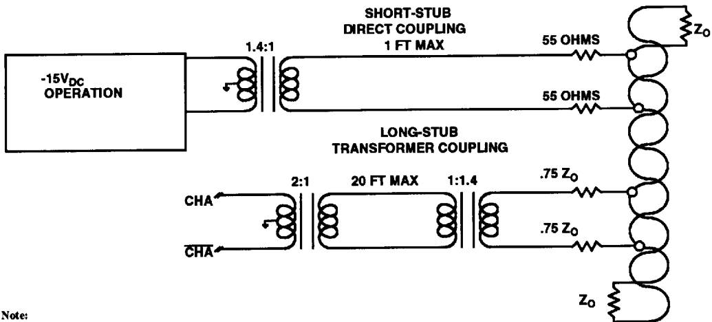
Figure 29a. S \mu MMIT LX15, XT15 Bus Coupling Configuration
