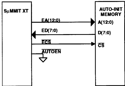
Figure 23a. Auto-Initialization System Configuration
