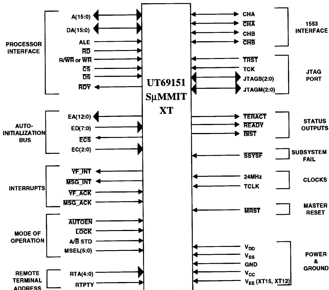
Figure 32. SμMMIT XT Functional Pin Diagram
