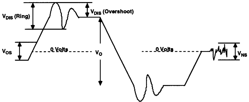
Figure 52. Transmitter Output Characteristics ( V_{DIS} , V_{OS} , V_{NS} , V_O )
