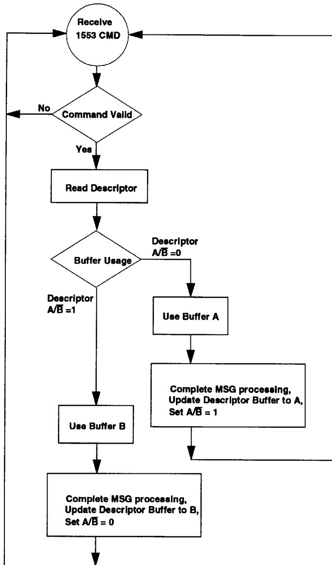
Figure 18. Ping-Pong Buffer Flow Chart
