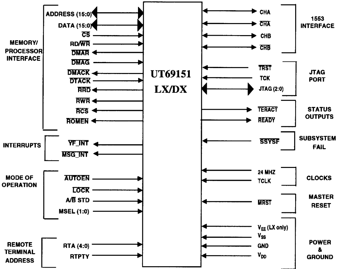
Figure 31. SμMMIT LX/DX Functional Pin Description
