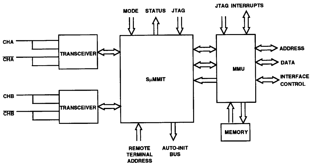
Figure 3. UT69151 S \mu MMIT XT Block Diagram
