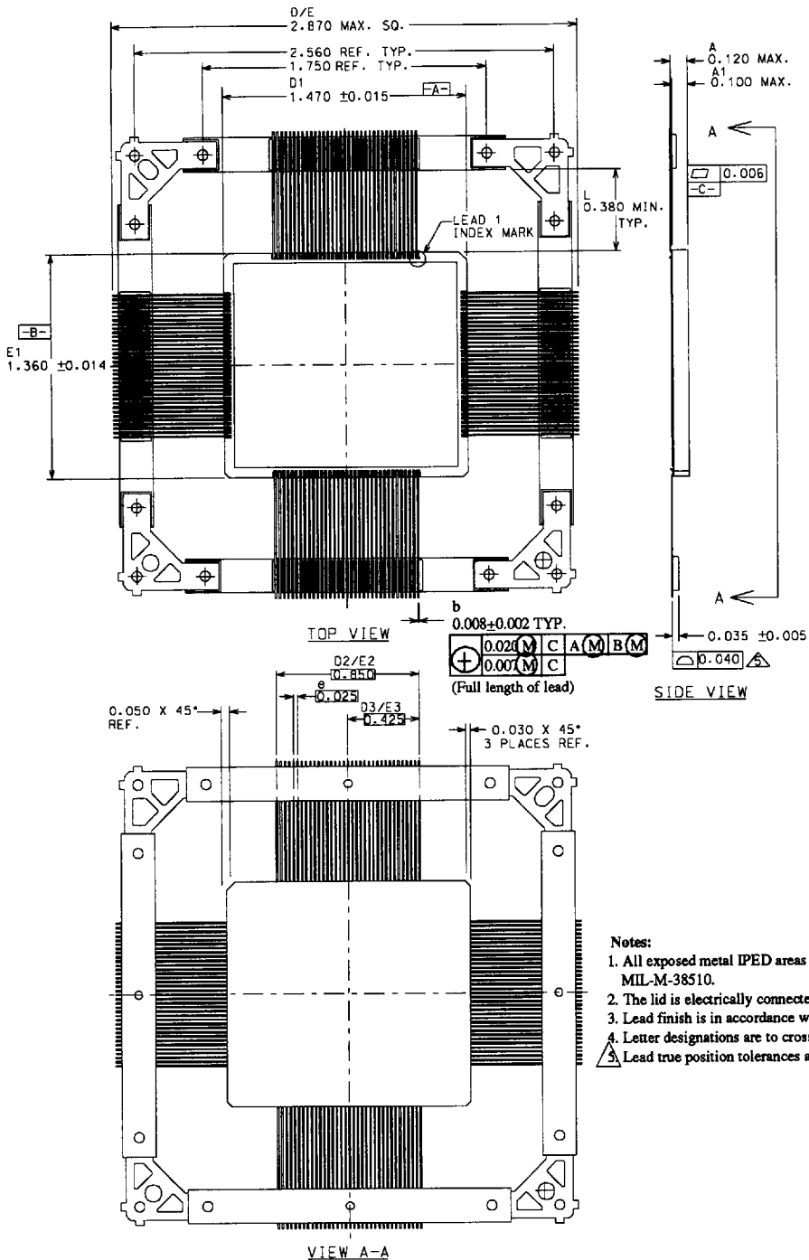
Figure 61. SμMMIT XT 140-Lead Flatpack
