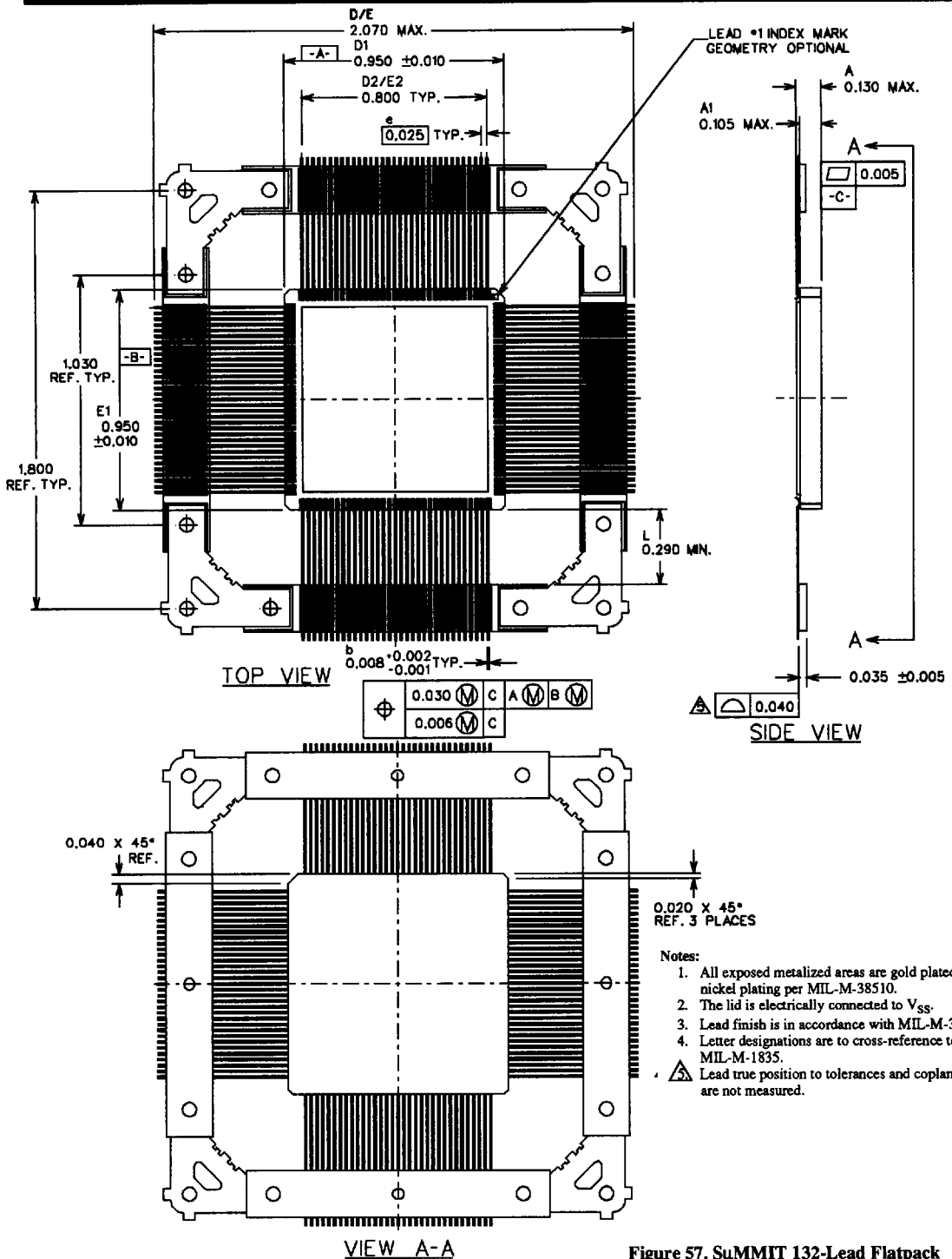
Figure 57. ΣμMMIT 132-Lead Flatpack
