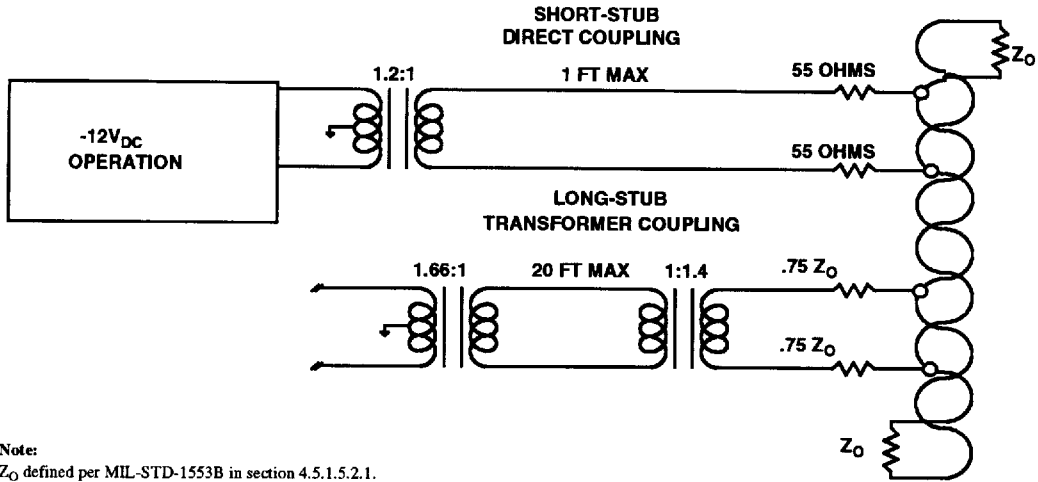
Figure 29b. SμMMIT LX12, XT12 Bus Coupling Configuration
