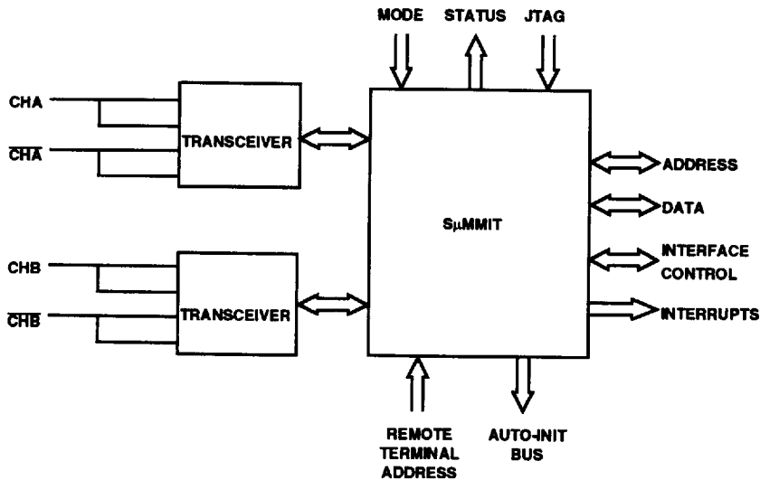
Figure 2. UT69151 S \mu MMIT LX/DX Block Diagram
