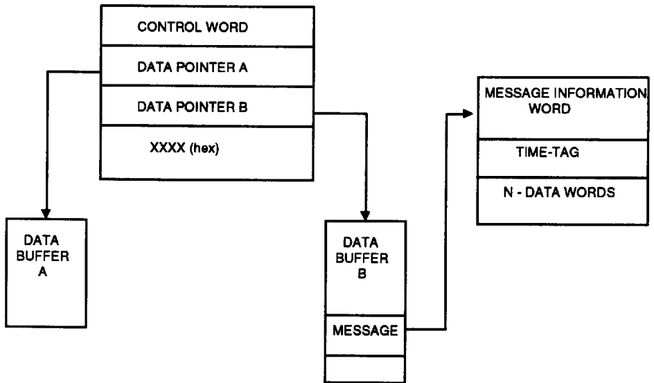
Figure 6. SRT Descriptor Block (Receive)
