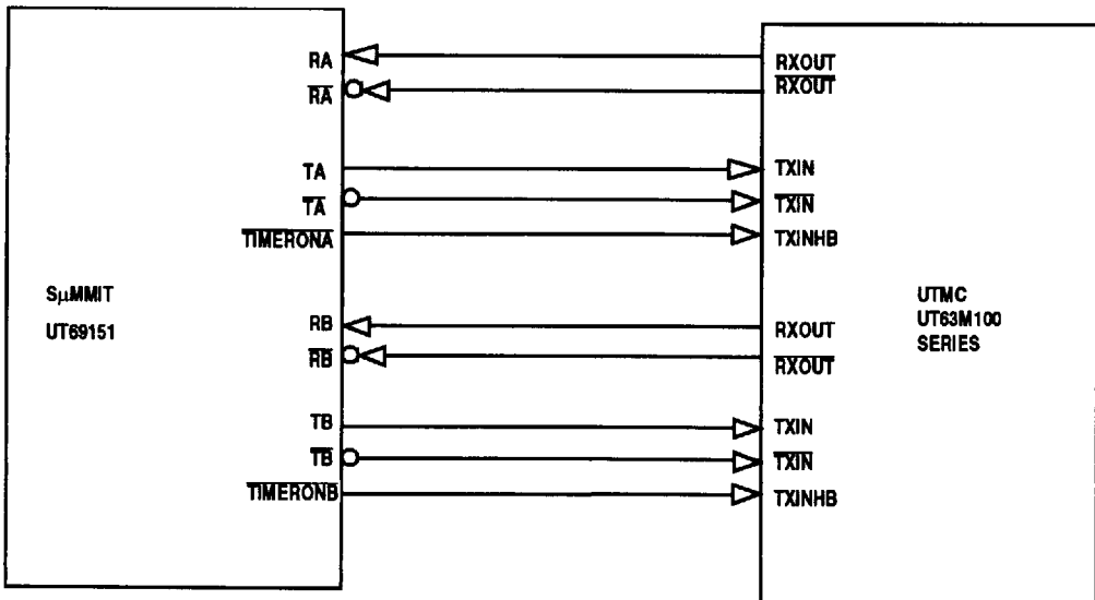
Figure 24b. S \mu MMIT Transceiver Interface Diagram
