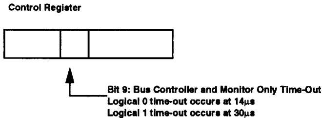
Figure 15. Programmable Bus Controller Time-Out
