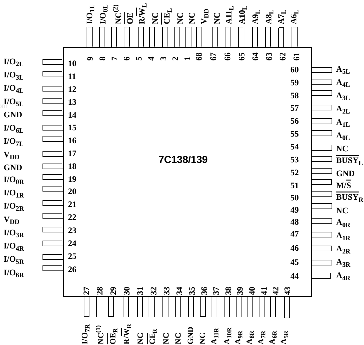
Figure 2a. DPRAM Pinout (68-Pin Flatpack) (top view)
