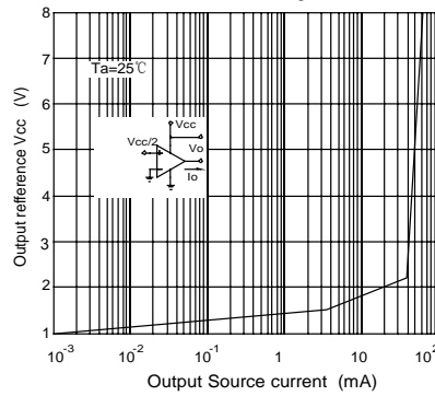
Fig.12 Current Limiting
