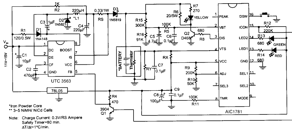
Fig. 3 Step-Down Converter
