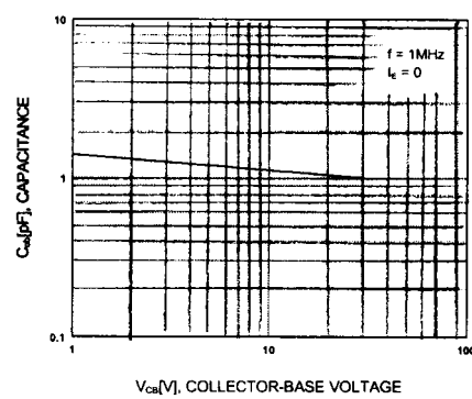
Figure 4. Output Capacitance
