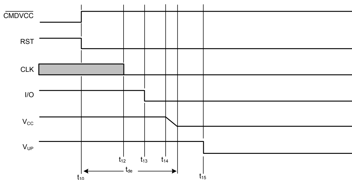
Fig.3 Deactivation Sequence
