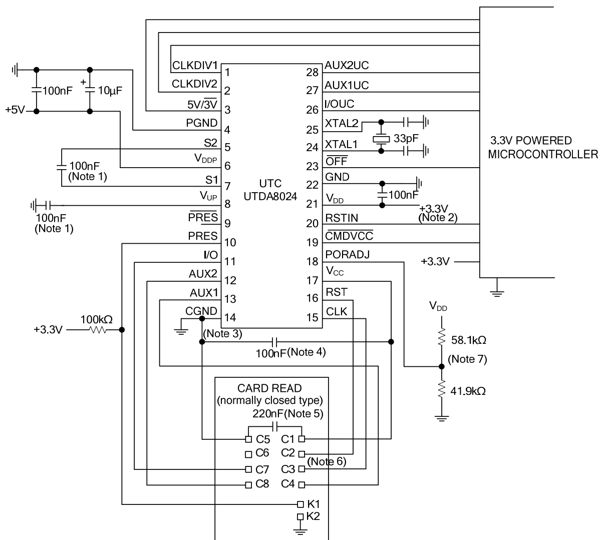
Fig. 6 Application Diagram.
