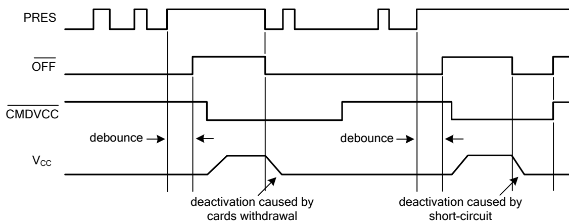
Fig. 4 Behaviour of \overline{\text{OFF}} , \overline{\text{CMDVCC}} , \overline{\text{PRES}} and V_{\text{CC}} .
