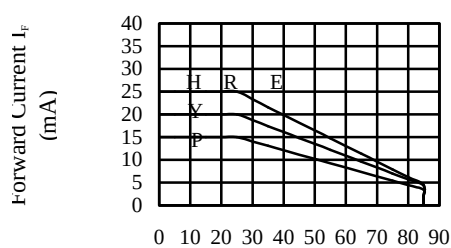
FIG.3 ALLOWABLE DC CURRENT VS. AMBIENT TEMPERATURE
