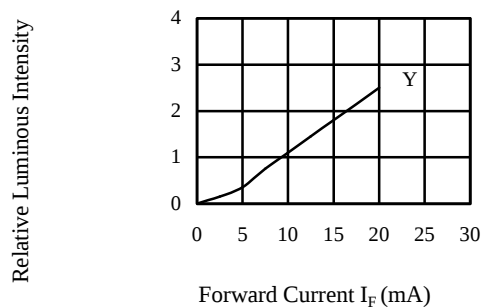
FIG.2-1 RELATIVE LUMINOUS INTENSITY VS. FORWARD CURRENT
