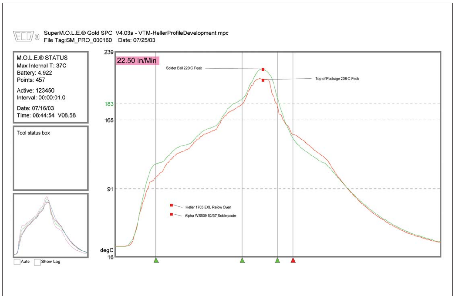
Figure 32—Thermal profile diagram
