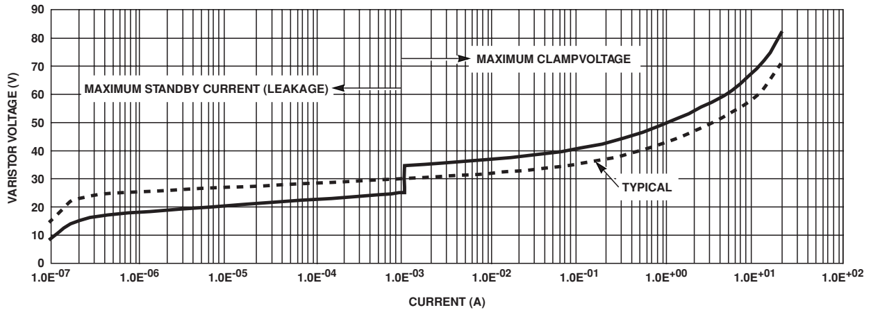
FIGURE 5. V-I CHARACTERISTICS
