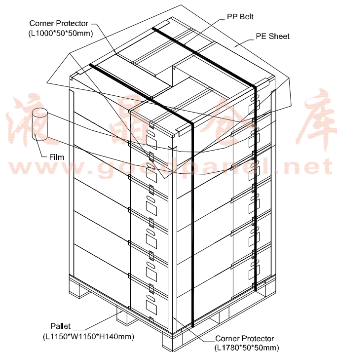
Figure.9-2 packing method
