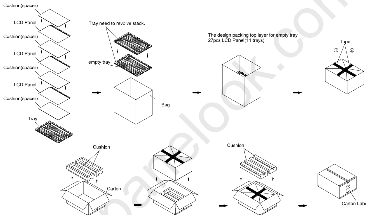
Figure.9-1 packing method
