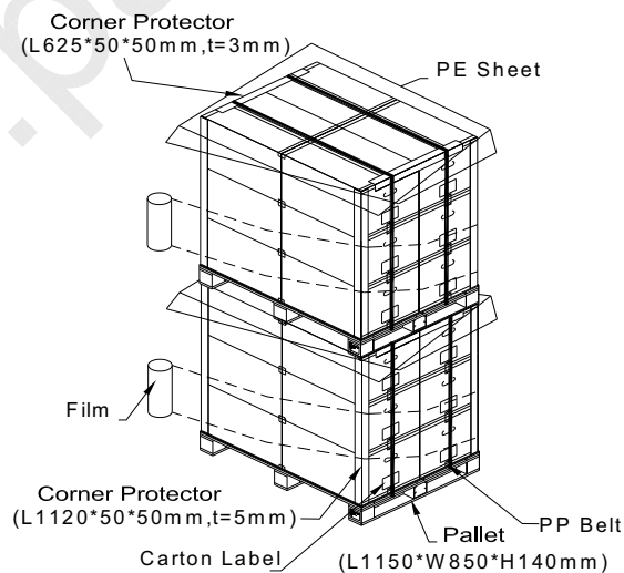
Figure 10-2 packing method
