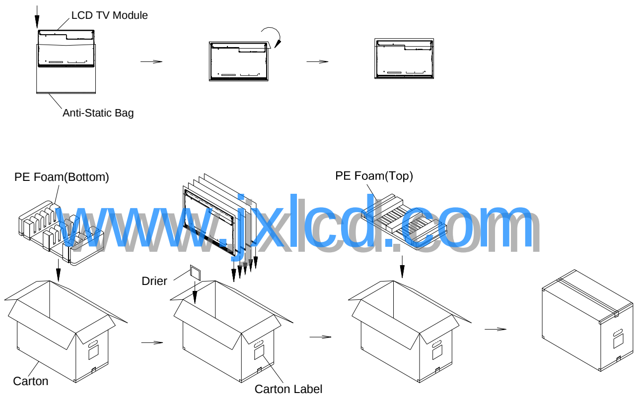
Figure.9-1 packing method
