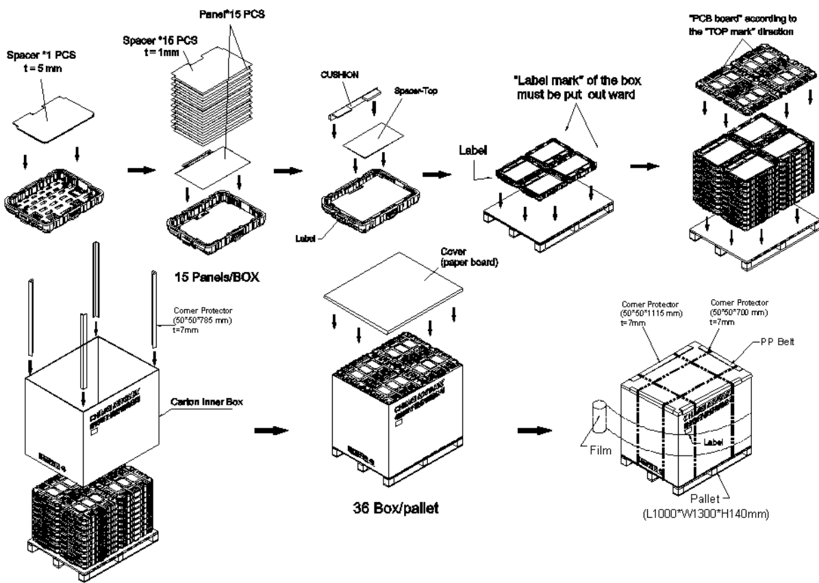
Figure.9-1 packing method
