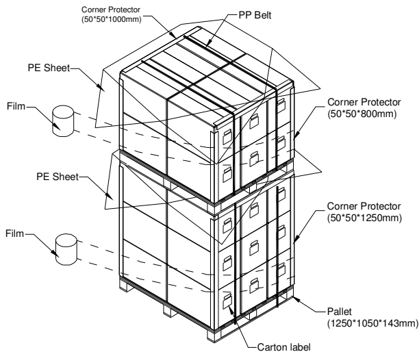
Figure. 8-2 Packing method
