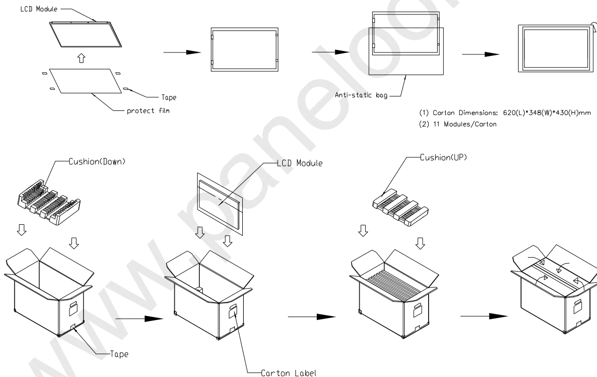
Figure. 8-1 Packing method
