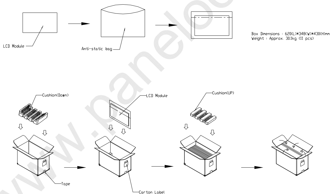
Figure. 7-1 Packing method
