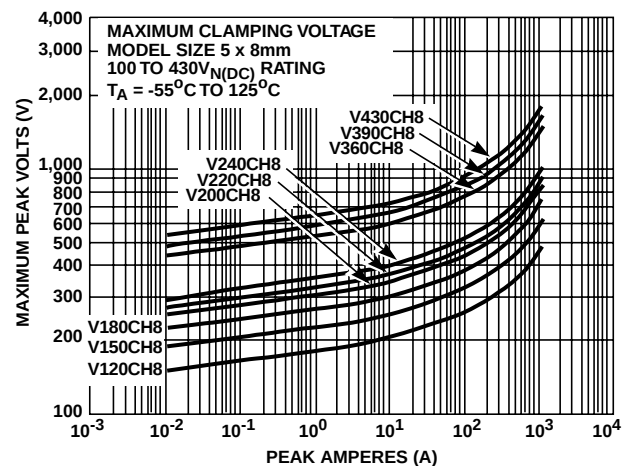
FIGURE 4. CLAMPING VOLTAGE FOR V120CH8 - V430CH8
