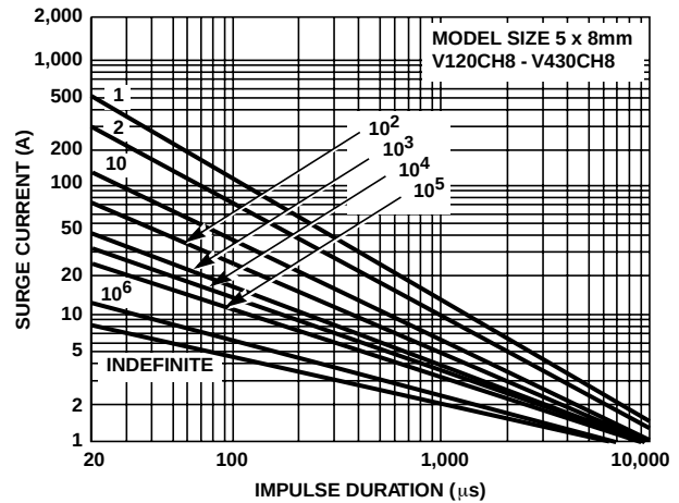
FIGURE 6. SURGE CURRENT RATING CURVES FOR V120CH8 - V430CH8
