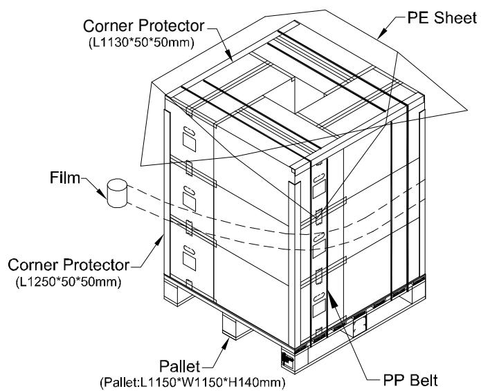
Figure. 9-2 packing method
