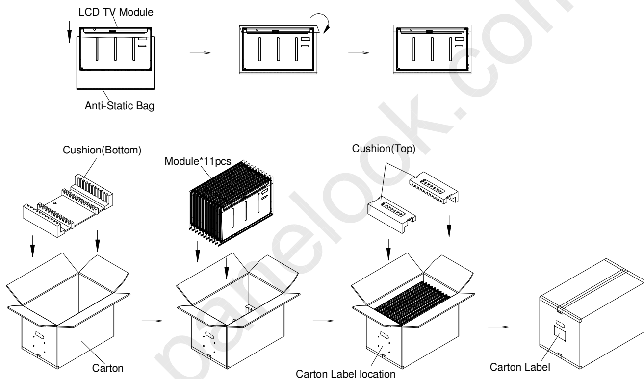
Figure.9-1 packing method
