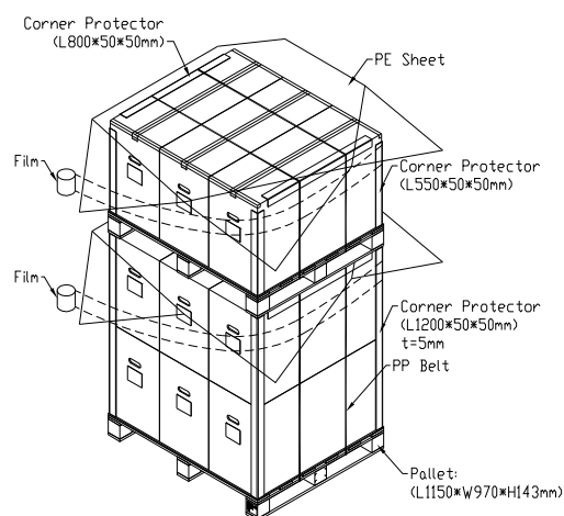
Figure.10.2 Packing method
