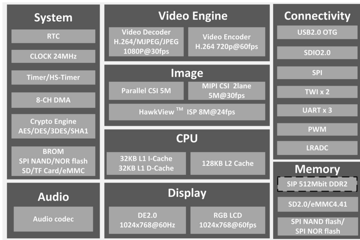
Figure 2-1. V3LP Block Diagram
