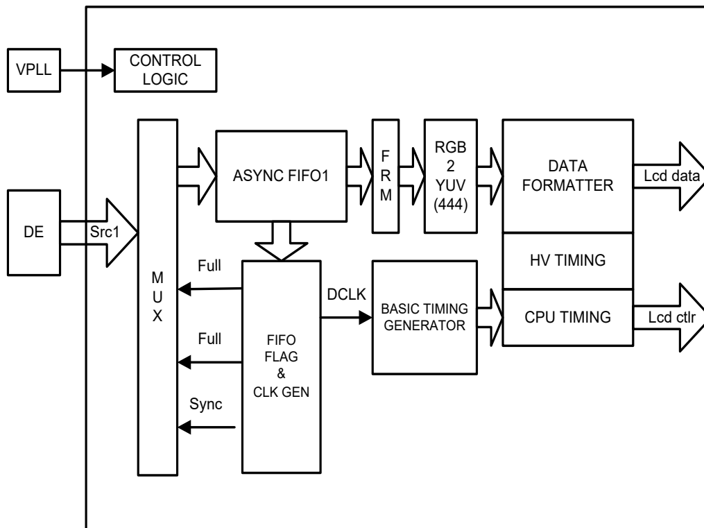
Figure 7-2. TCON Block Diagram
