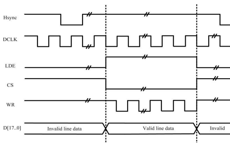
Figure 7-7. Lcd_CPUI/F Timing
