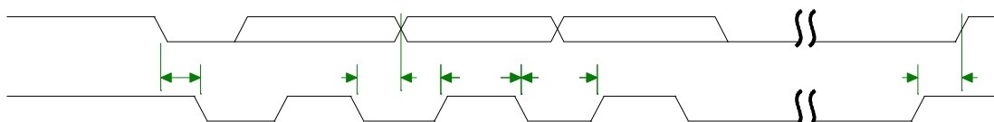
Figure 8-1 . TWI Timing Diagram
