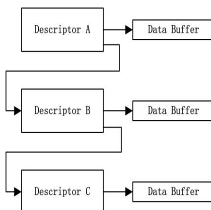
Figure 5-3. SD/MMC IDMAC Descriptor and Buffer
