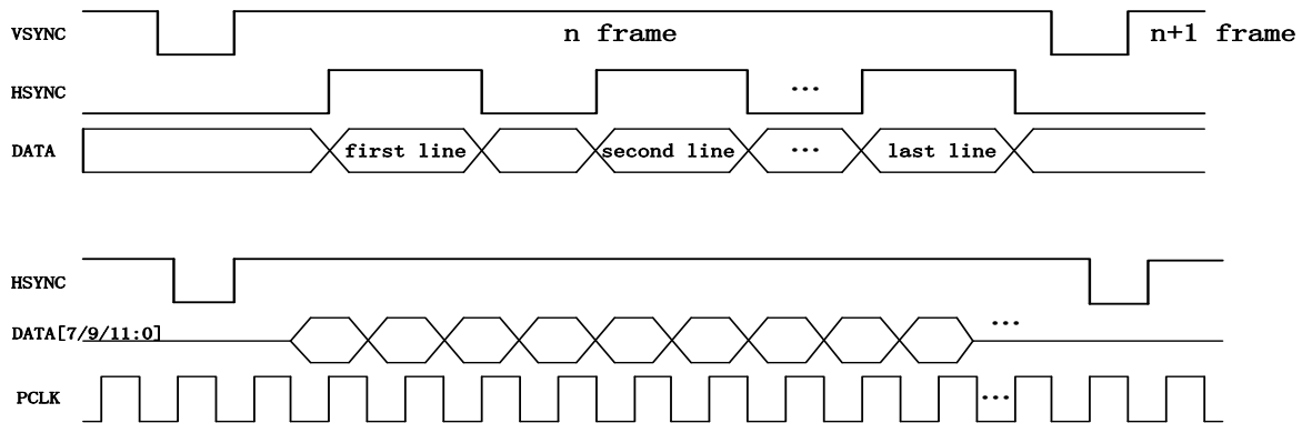
Figure 6-3. 8/10/12-bit CMOS Sensor Interface Timing (clock rising edge sample.vsync valid = positive,hsync valid = positive)
