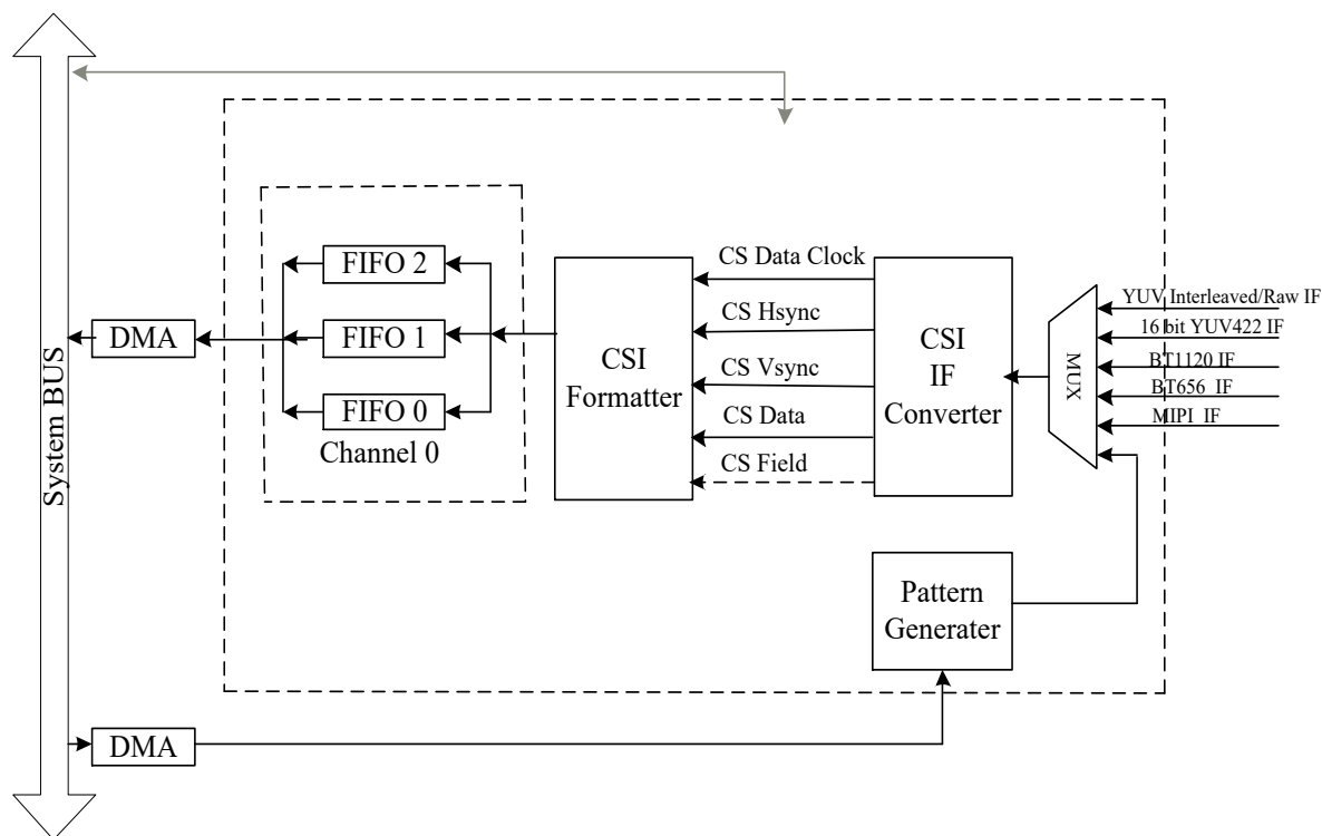
Figure 6-1. CSI Block Diagram
