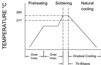
Figure 1. Re-flow Soldering
