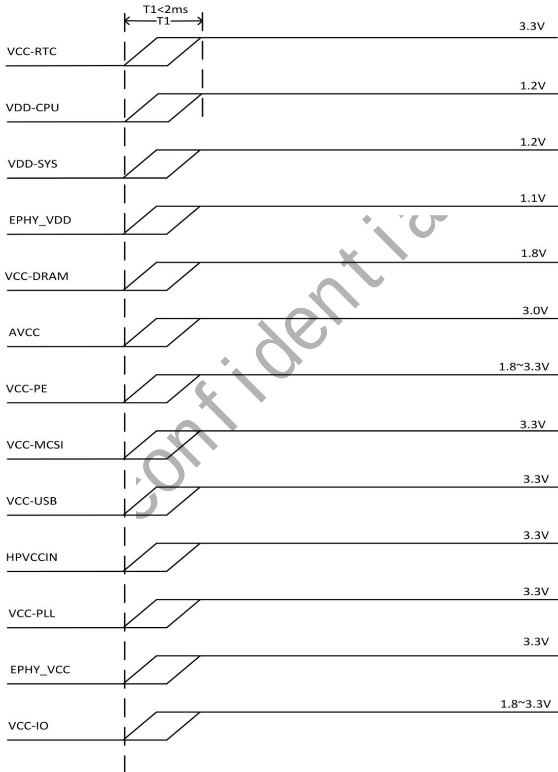
Figure 9-1. Power On Sequence
