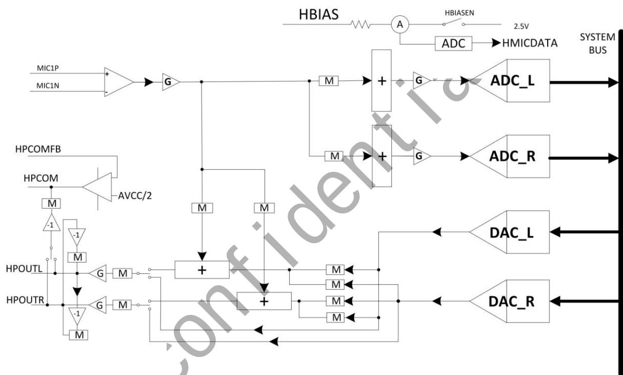
Figure 4-10. Analog Data Path Diagram
