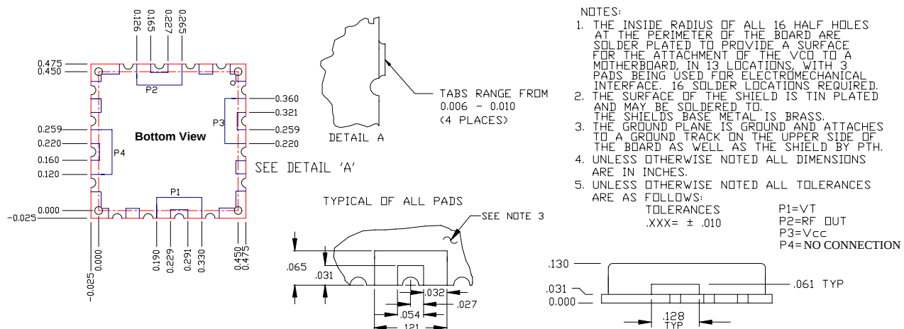
PHYSICAL DIMENSIONS
