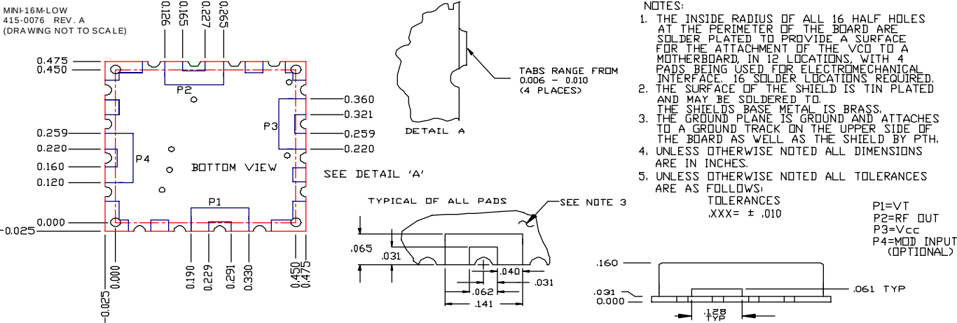
PHYSICAL DIMENSIONS
